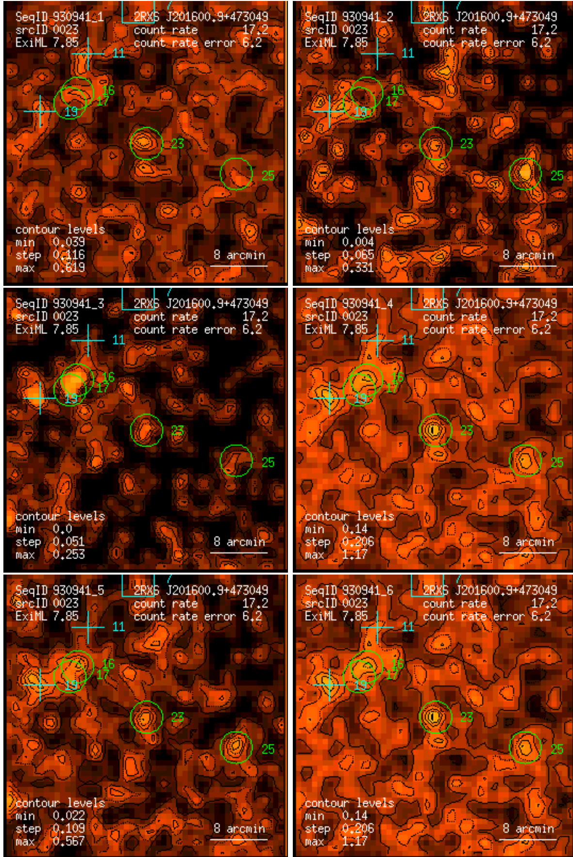
Figure 23: RASS 930941: detection 0023: band rate images, Gaussian filter: (1) PSPC channels 11 – 41, (2) 52 – 90, (3) 91 – 201, (4) 11 – 235, (5) 52 – 201, (6) 11 – 201. Broad band rates in counts/ks. Band rate contour levels in counts/ks/arcmin 2 .
