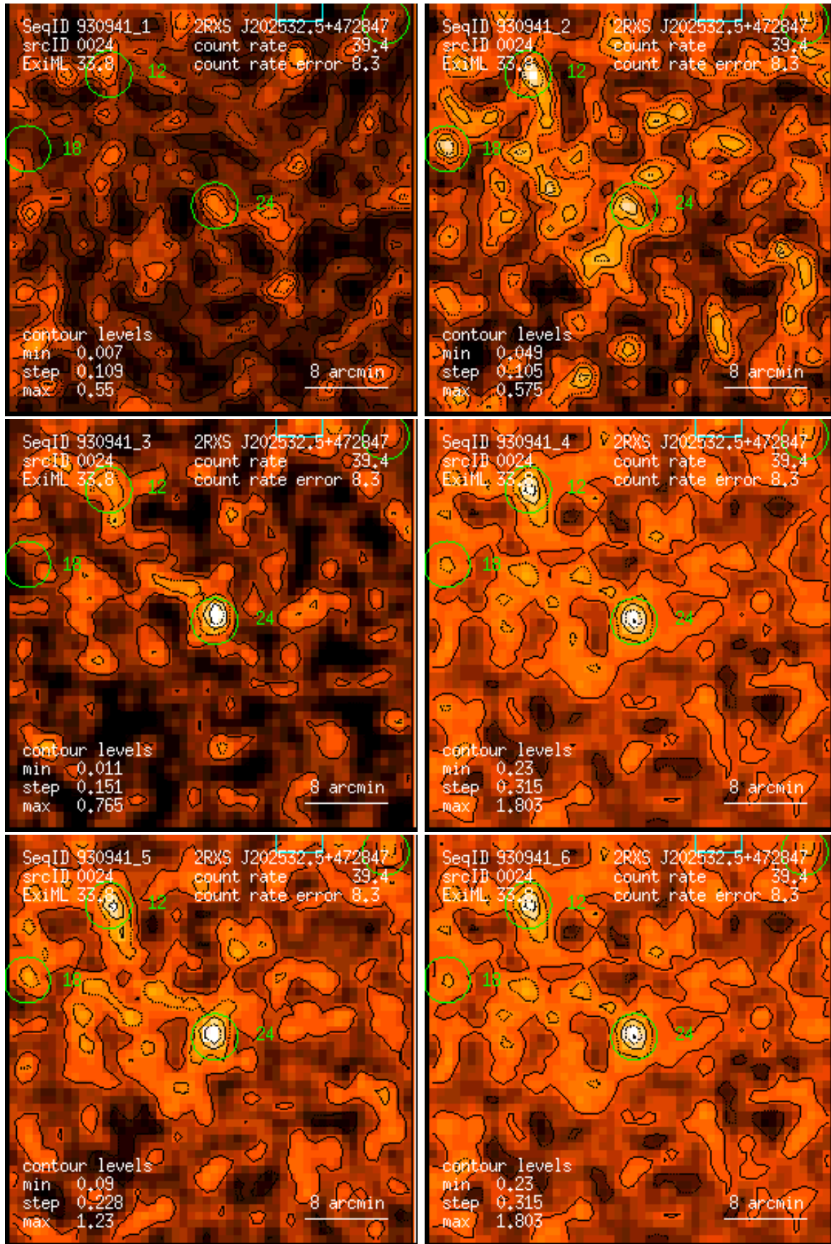
Figure 24: RASS 930941: detection 0024: band rate images, Gaussian filter: (1) PSPC channels 11 – 41, (2) 52 – 90, (3) 91 – 201, (4) 11 – 235, (5) 52 – 201, (6) 11 – 201. Broad band rates in counts/ks. Band rate contour levels in counts/ks/arcmin 2 .
