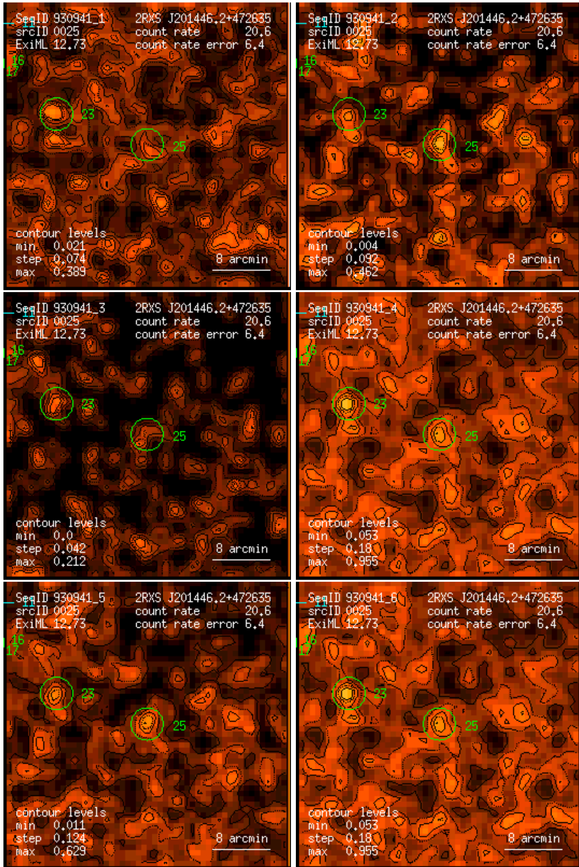
Figure 25: RASS 930941: detection 0025: band rate images, Gaussian filter: (1) PSPC channels 11 – 41, (2) 52 – 90, (3) 91 – 201, (4) 11 – 235, (5) 52 – 201, (6) 11 – 201. Broad band rates in counts/ks. Band rate contour levels in counts/ks/arcmin 2 .
