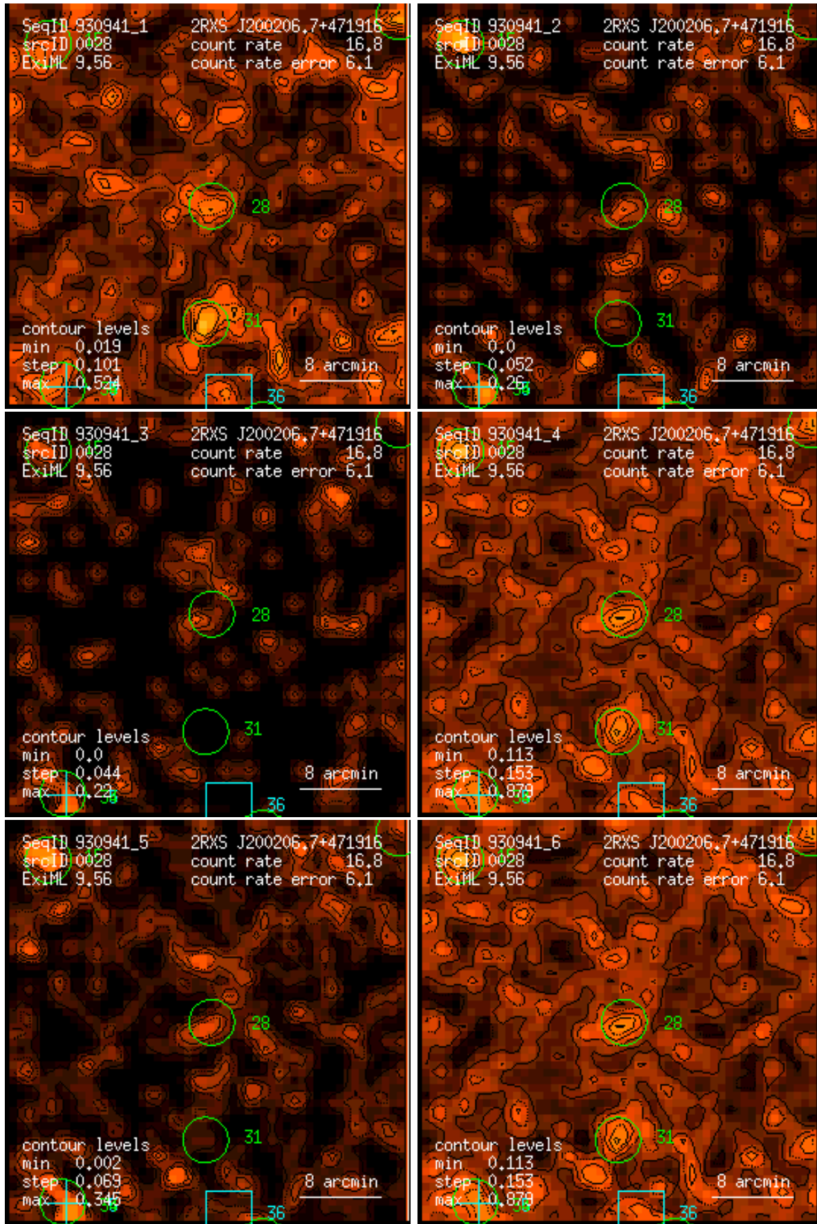
Figure 28: RASS 930941: detection 0028: band rate images, Gaussian filter: (1) PSPC channels 11 – 41, (2) 52 – 90, (3) 91 – 201, (4) 11 – 235, (5) 52 – 201, (6) 11 – 201. Broad band rates in counts/ks. Band rate contour levels in counts/ks/arcmin 2 .
