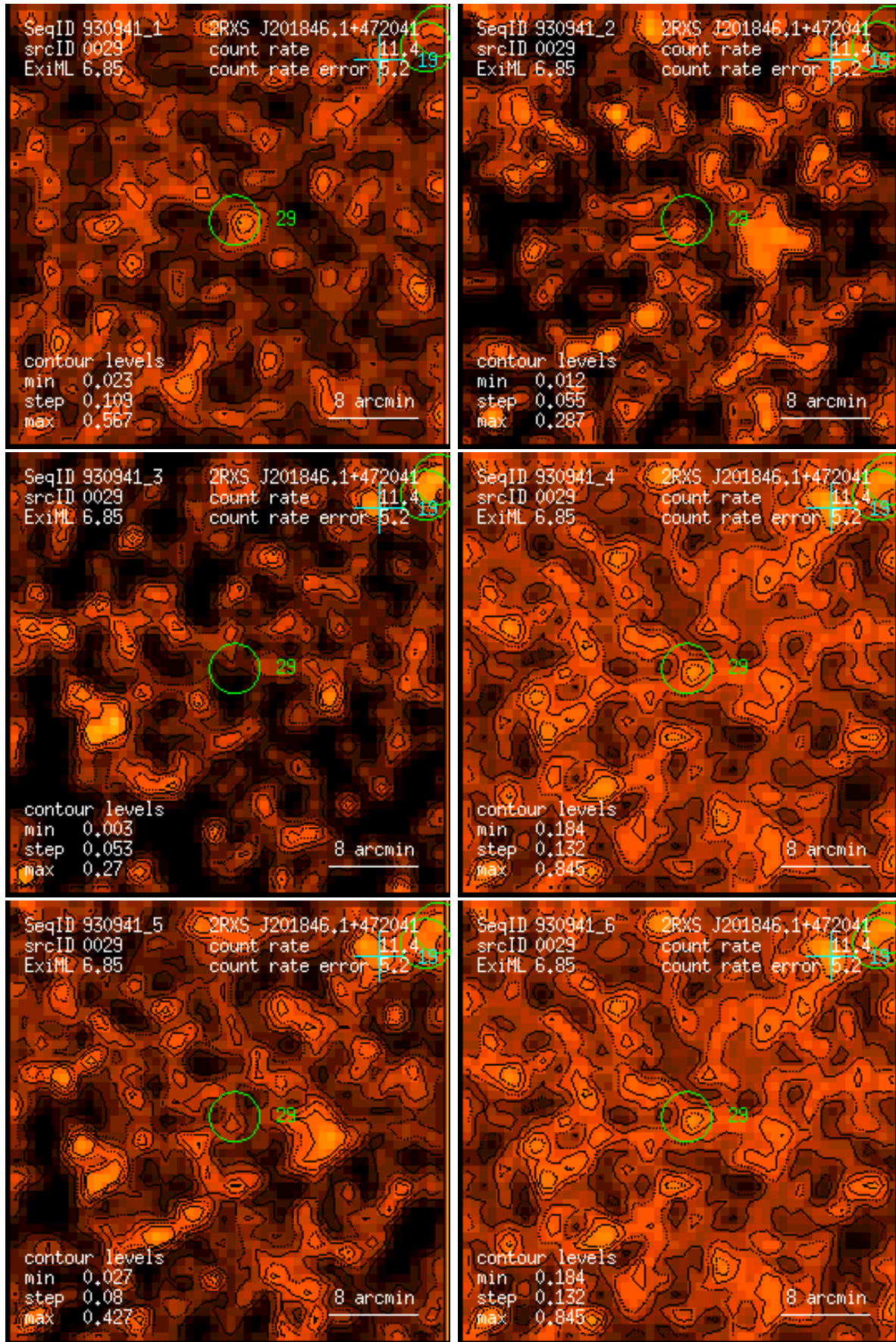
Figure 29: RASS 930941: detection 0029: band rate images, Gaussian filter: (1) PSPC channels 11 – 41, (2) 52 – 90, (3) 91 – 201, (4) 11 – 235, (5) 52 – 201, (6) 11 – 201. Broad band rates in counts/ks. Band rate contour levels in counts/ks/arcmin 2 .
