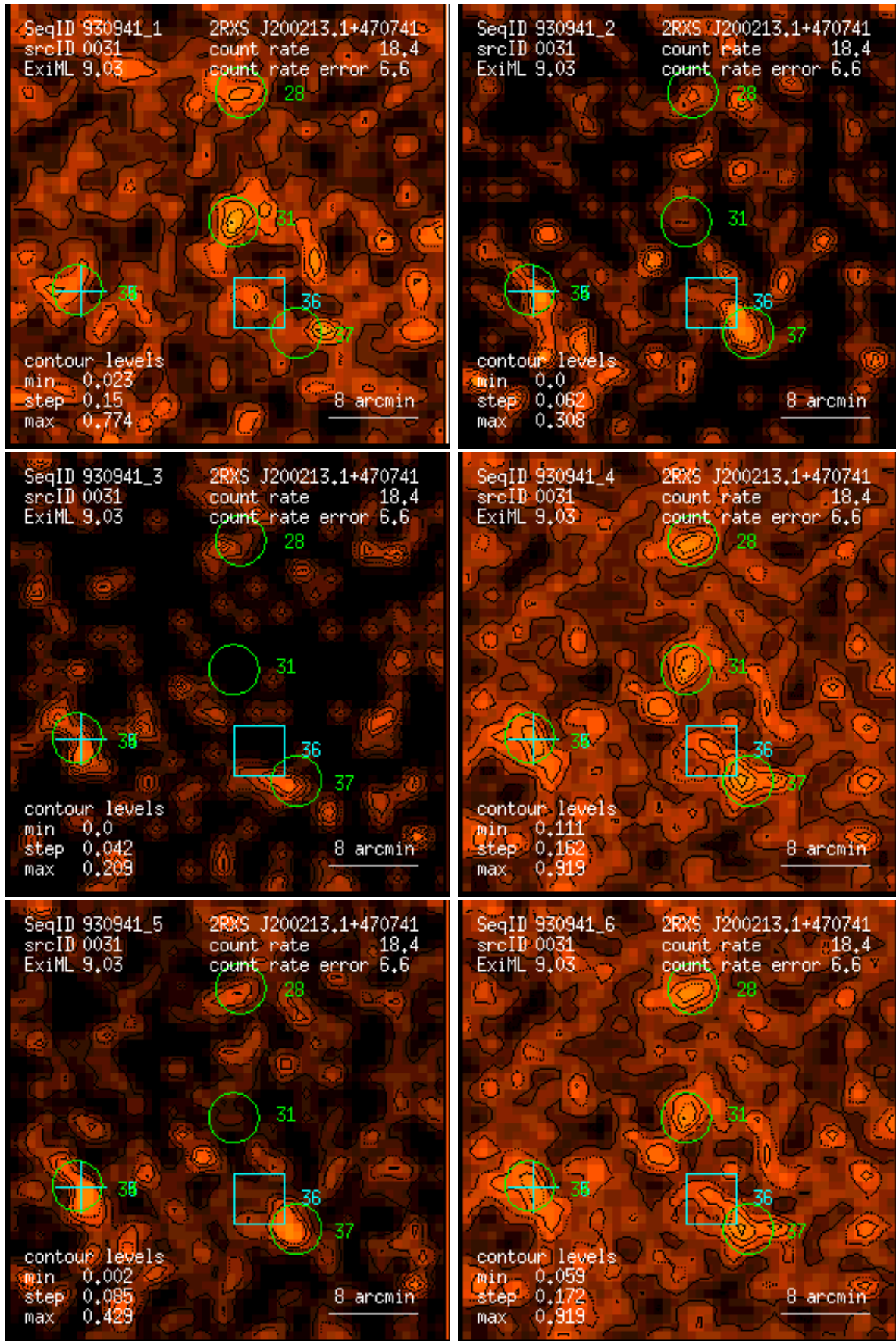
Figure 31: RASS 930941: detection 0031: band rate images, Gaussian filter: (1) PSPC channels 11 – 41, (2) 52 – 90, (3) 91 – 201, (4) 11 – 235, (5) 52 – 201, (6) 11 – 201. Broad band rates in counts/ks. Band rate contour levels in counts/ks/arcmin 2 .
