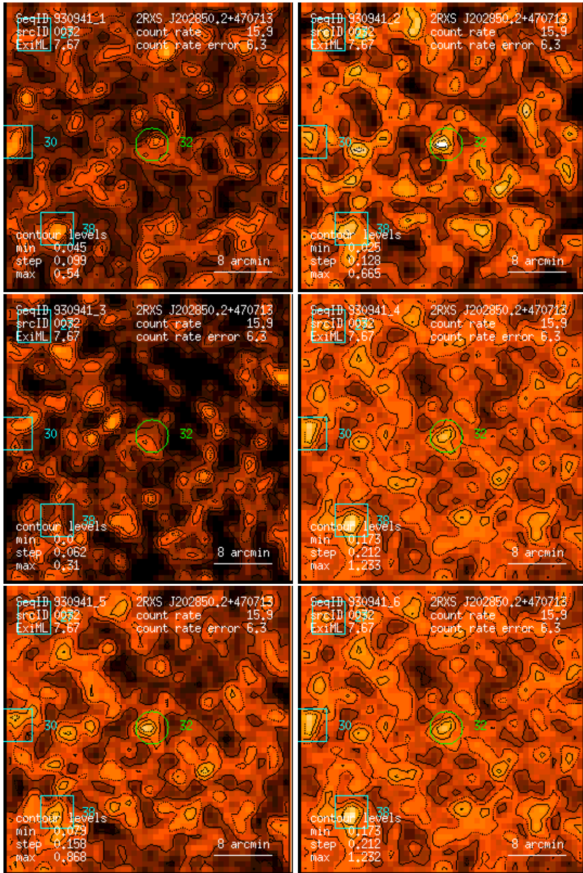
Figure 32: RASS 930941: detection 0032: band rate images, Gaussian filter: (1) PSPC channels 11 – 41, (2) 52 – 90, (3) 91 – 201, (4) 11 – 235, (5) 52 – 201, (6) 11 – 201. Broad band rates in counts/ks. Band rate contour levels in counts/ks/arcmin 2 .
