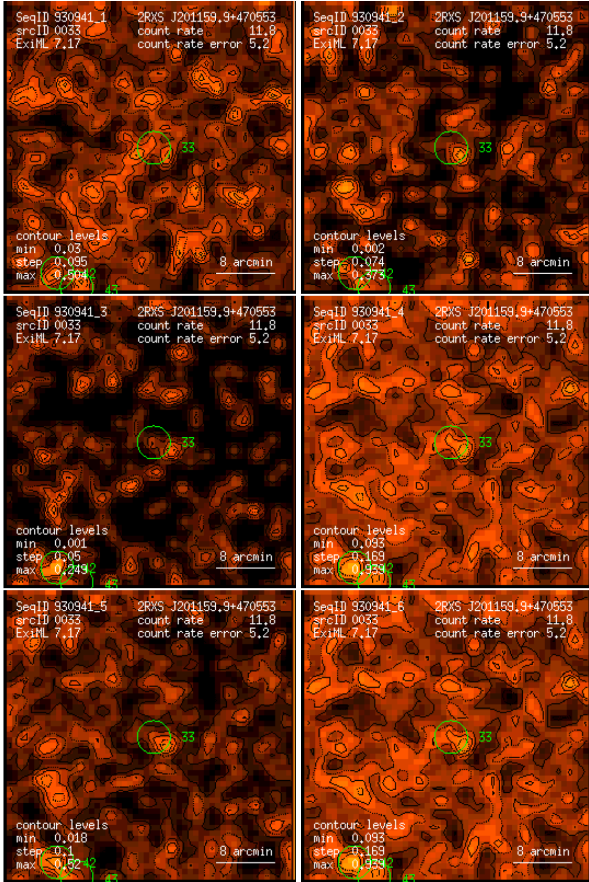
Figure 33: RASS 930941: detection 0033: band rate images, Gaussian filter: (1) PSPC channels 11 – 41, (2) 52 – 90, (3) 91 – 201, (4) 11 – 235, (5) 52 – 201, (6) 11 – 201. Broad band rates in counts/ks. Band rate contour levels in counts/ks/arcmin 2 .
