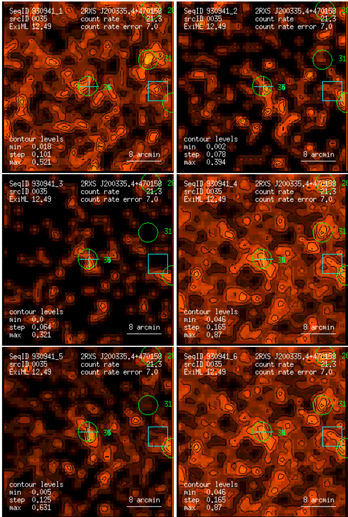
Figure 35: RASS 930941: detection 0035: band rate images, Gaussian filter: (1) PSPC channels 11 – 41, (2) 52 – 90, (3) 91 – 201, (4) 11 – 235, (5) 52 – 201, (6) 11 – 201. Broad band rates in counts/ks. Band rate contour levels in counts/ks/arcmin 2 .
