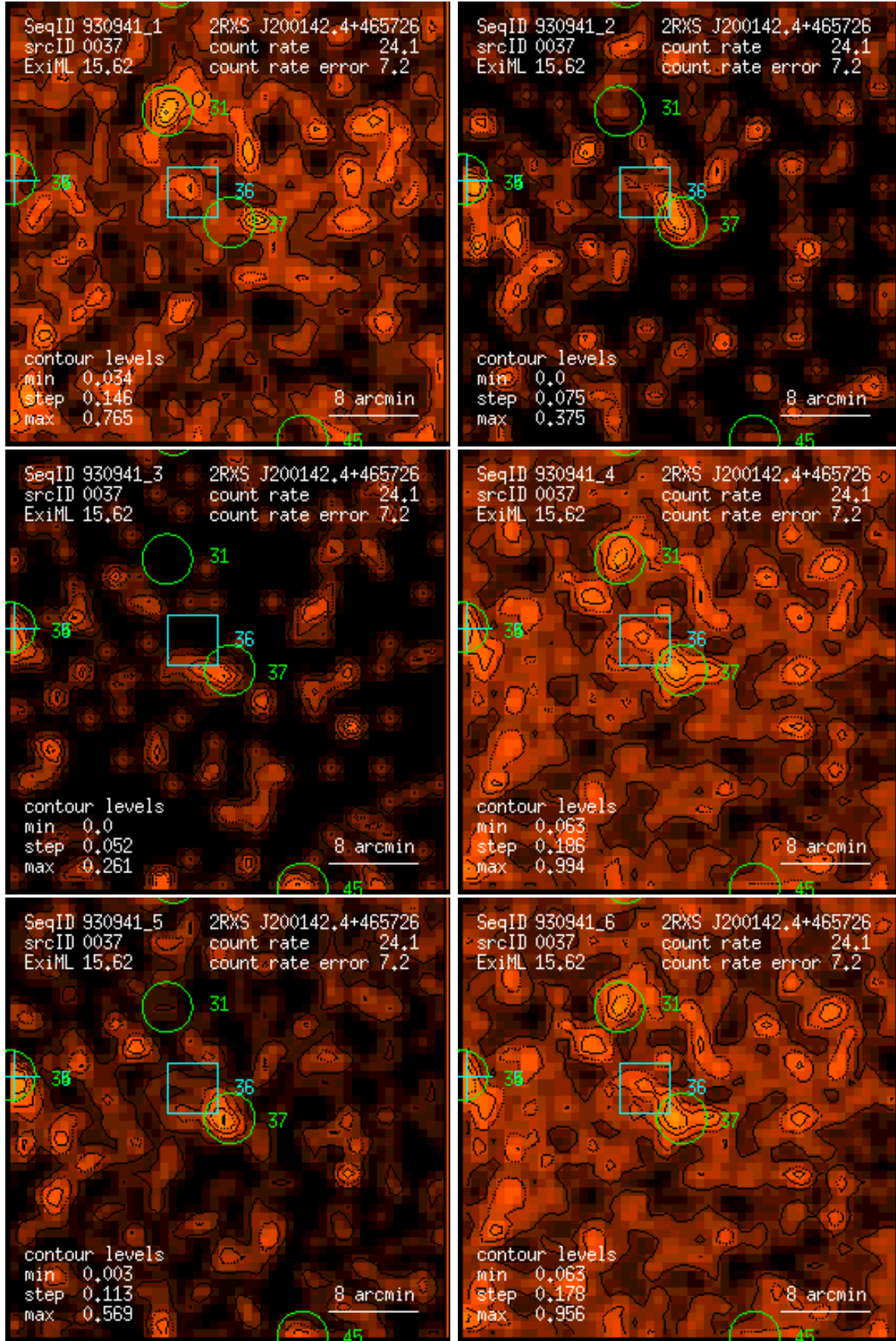
Figure 37: RASS 930941: detection 0037: band rate images, Gaussian filter: (1) PSPC channels 11 – 41, (2) 52 – 90, (3) 91 – 201, (4) 11 – 235, (5) 52 – 201, (6) 11 – 201. Broad band rates in counts/ks. Band rate contour levels in counts/ks/arcmin 2 .
