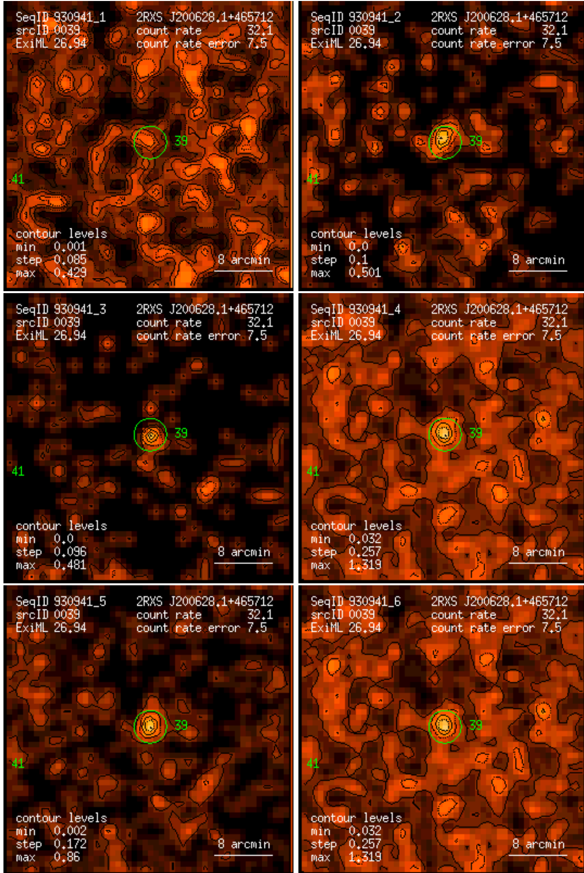
Figure 39: RASS 930941: detection 0039: band rate images, Gaussian filter: (1) PSPC channels 11 – 41, (2) 52 – 90, (3) 91 – 201, (4) 11 – 235, (5) 52 – 201, (6) 11 – 201. Broad band rates in counts/ks. Band rate contour levels in counts/ks/arcmin 2 .
