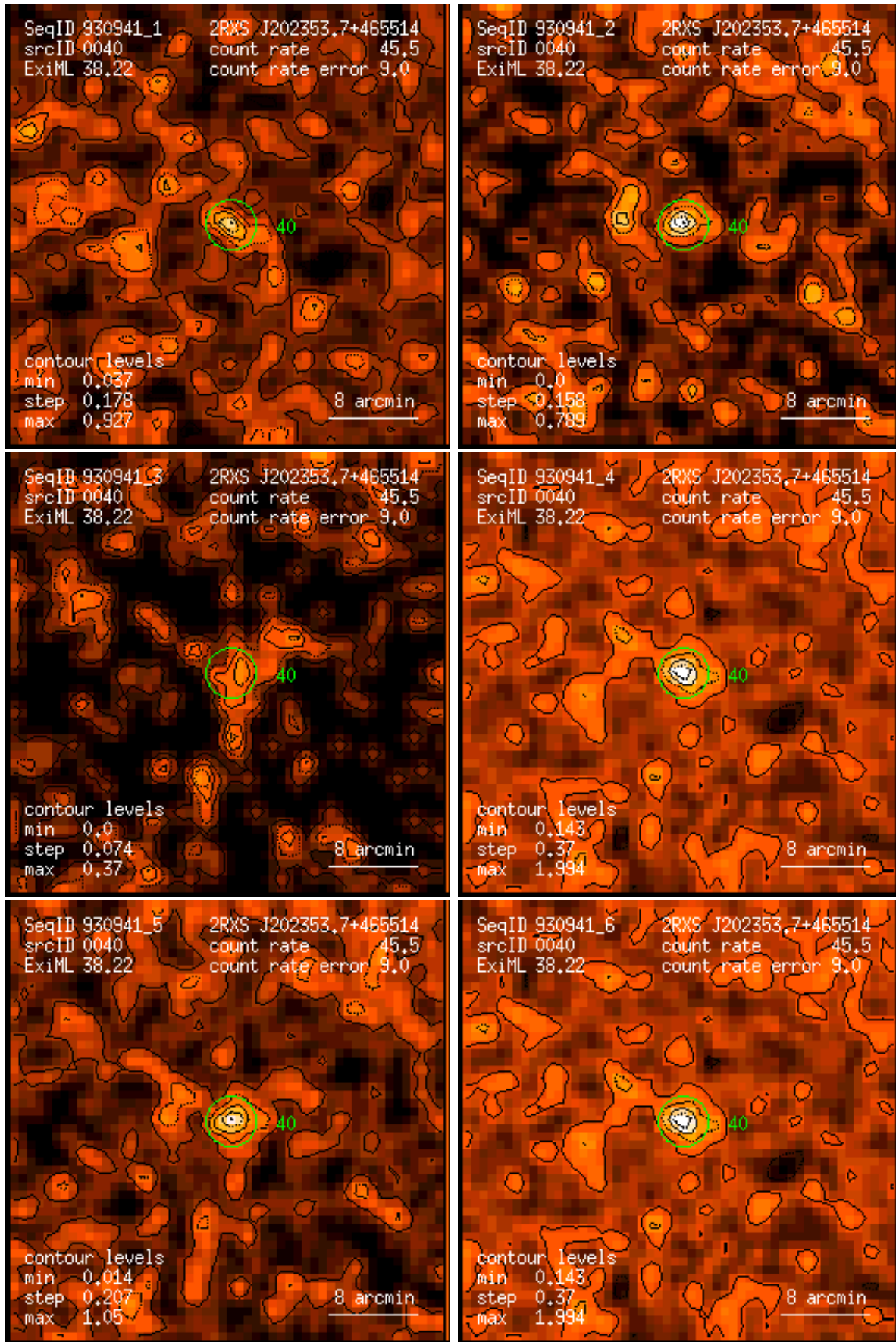
Figure 40: RASS 930941: detection 0040: band rate images, Gaussian filter: (1) PSPC channels 11 – 41, (2) 52 – 90, (3) 91 – 201, (4) 11 – 235, (5) 52 – 201, (6) 11 – 201. Broad band rates in counts/ks. Band rate contour levels in counts/ks/arcmin 2 .
