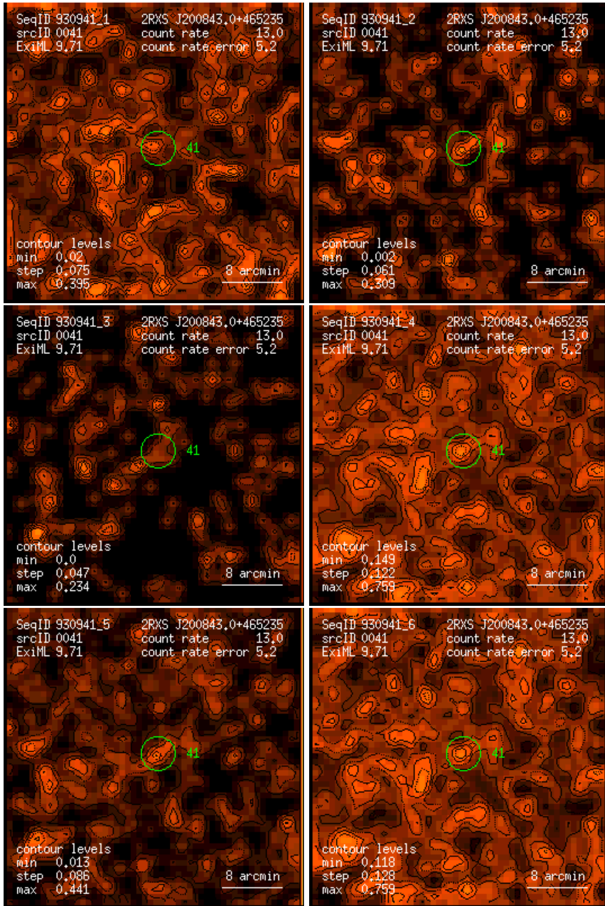
Figure 41: RASS 930941: detection 0041: band rate images, Gaussian filter: (1) PSPC channels 11 – 41, (2) 52 – 90, (3) 91 – 201, (4) 11 – 235, (5) 52 – 201, (6) 11 – 201. Broad band rates in counts/ks. Band rate contour levels in counts/ks/arcmin 2 .
