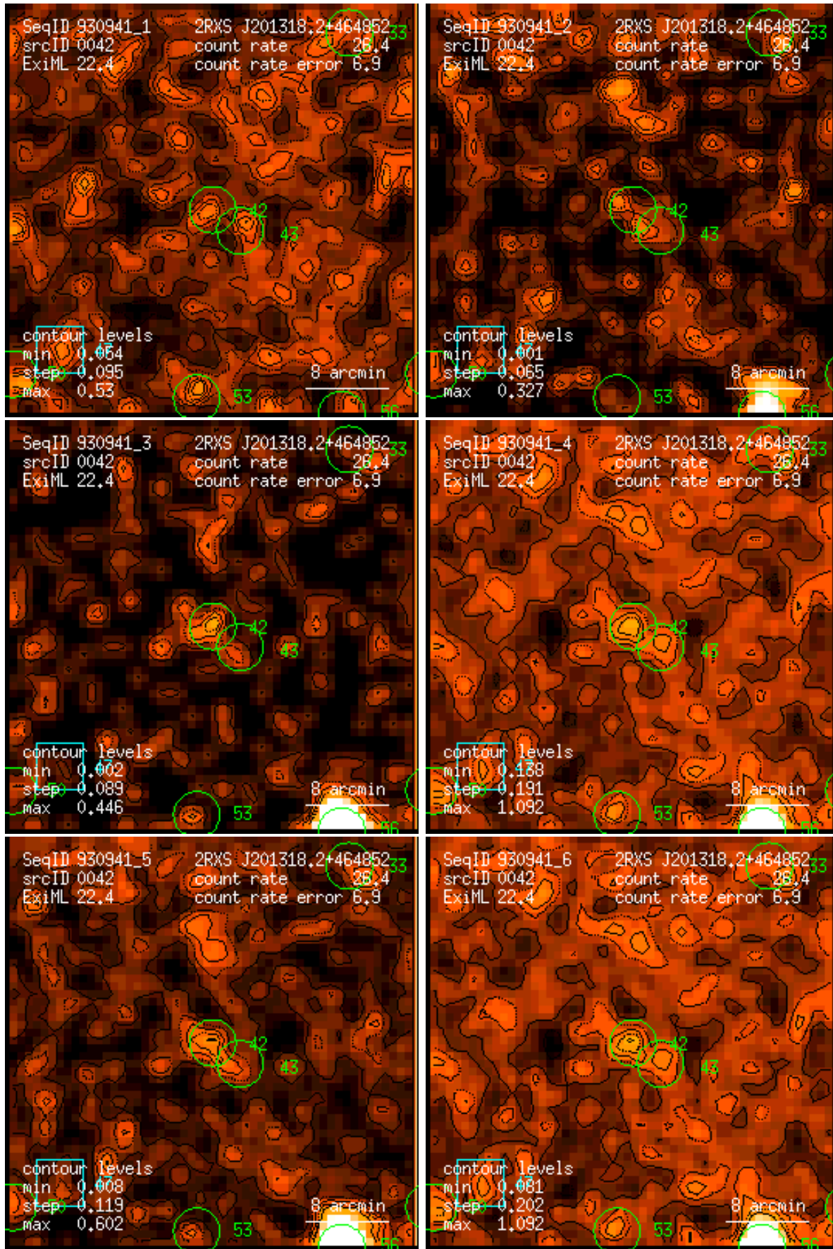
Figure 42: RASS 930941: detection 0042: band rate images, Gaussian filter: (1) PSPC channels 11 – 41, (2) 52 – 90, (3) 91 – 201, (4) 11 – 235, (5) 52 – 201, (6) 11 – 201. Broad band rates in counts/ks. Band rate contour levels in counts/ks/arcmin 2 .
