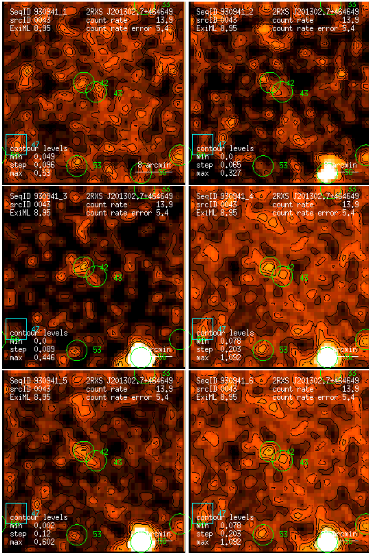
Figure 43: RASS 930941: detection 0043: band rate images, Gaussian filter: (1) PSPC channels 11 – 41, (2) 52 – 90, (3) 91 – 201, (4) 11 – 235, (5) 52 – 201, (6) 11 – 201. Broad band rates in counts/ks. Band rate contour levels in counts/ks/arcmin 2 .
