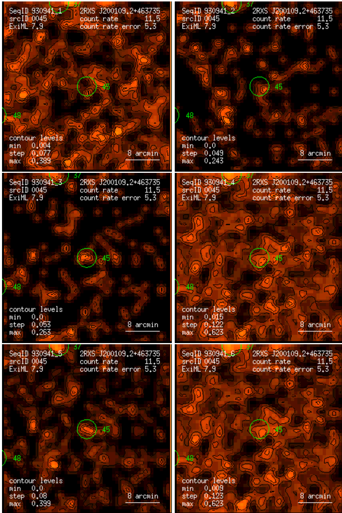
Figure 45: RASS 930941: detection 0045: band rate images, Gaussian filter: (1) PSPC channels 11 – 41, (2) 52 – 90, (3) 91 – 201, (4) 11 – 235, (5) 52 – 201, (6) 11 – 201. Broad band rates in counts/ks. Band rate contour levels in counts/ks/arcmin 2 .
