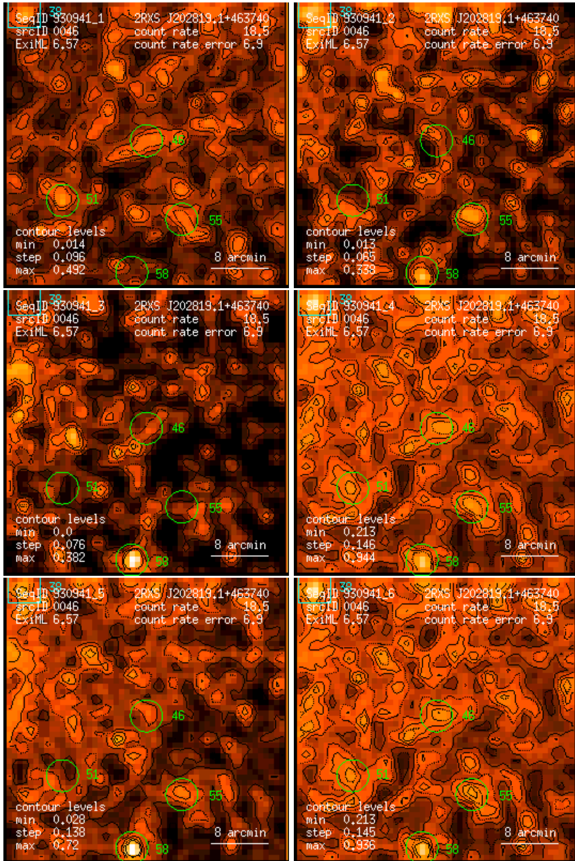
Figure 46: RASS 930941: detection 0046: band rate images, Gaussian filter: (1) PSPC channels 11 – 41, (2) 52 – 90, (3) 91 – 201, (4) 11 – 235, (5) 52 – 201, (6) 11 – 201. Broad band rates in counts/ks. Band rate contour levels in counts/ks/arcmin 2 .
