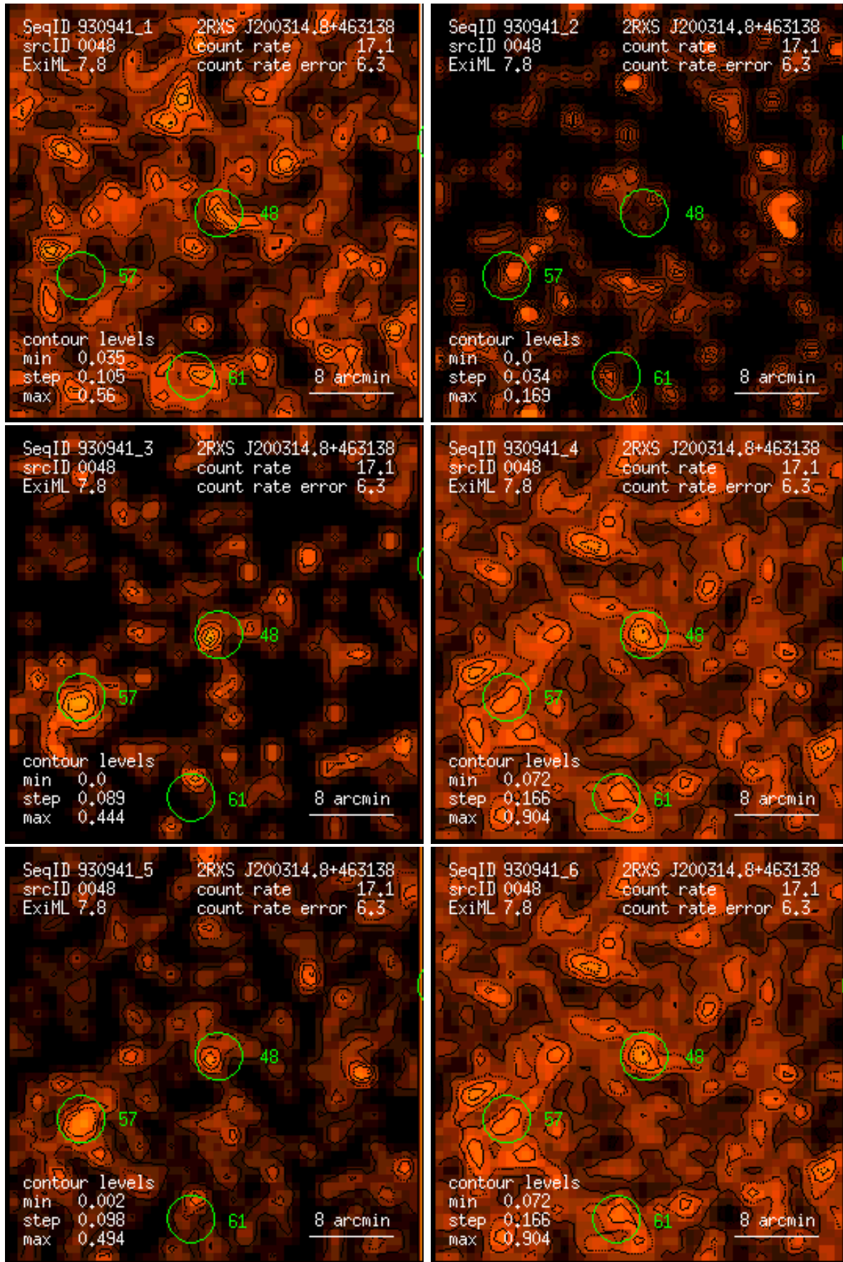
Figure 48: RASS 930941: detection 0048: band rate images, Gaussian filter: (1) PSPC channels 11 – 41, (2) 52 – 90, (3) 91 – 201, (4) 11 – 235, (5) 52 – 201, (6) 11 – 201. Broad band rates in counts/ks. Band rate contour levels in counts/ks/arcmin 2 .
