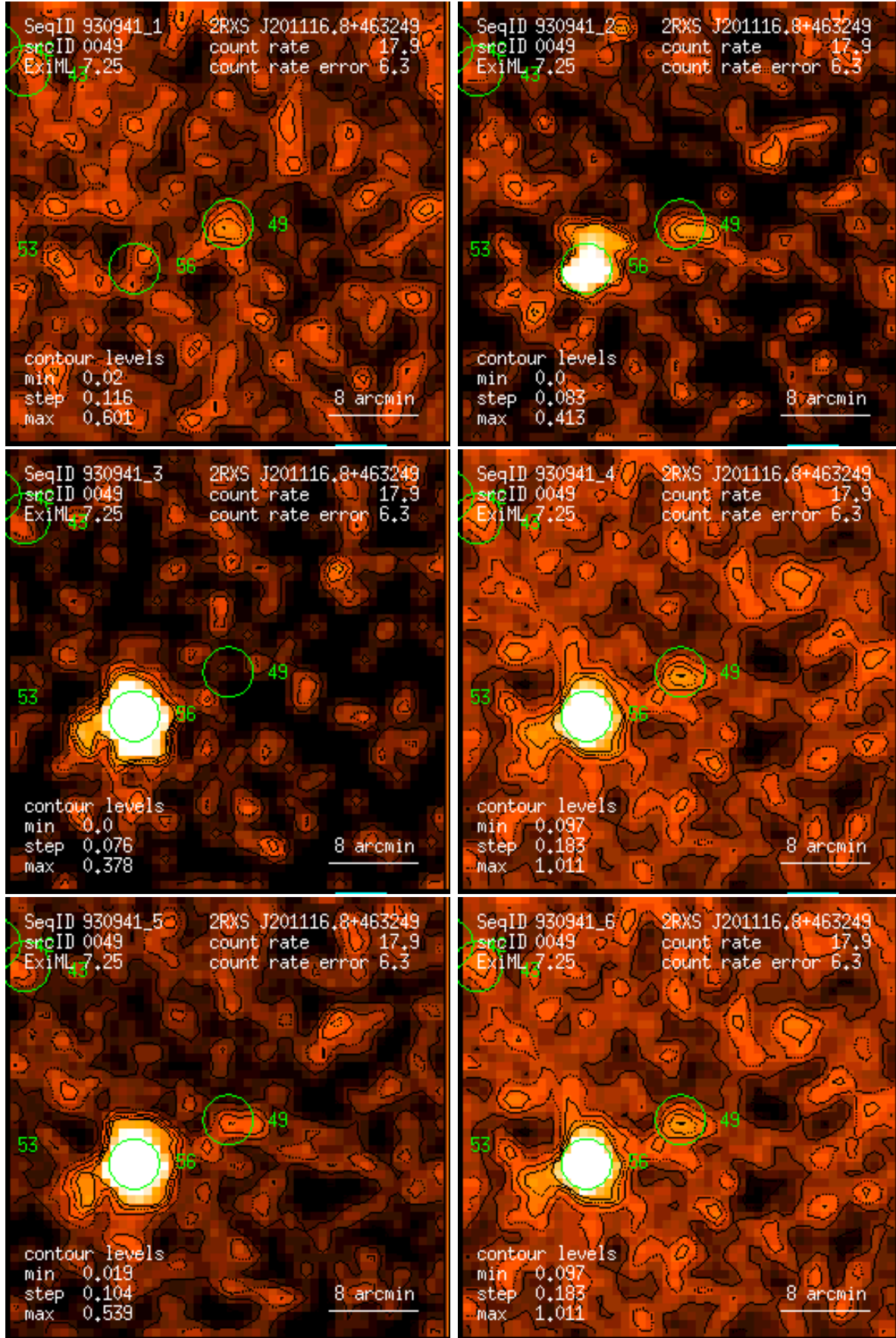
Figure 49: RASS 930941: detection 0049: band rate images, Gaussian filter: (1) PSPC channels 11 – 41, (2) 52 – 90, (3) 91 – 201, (4) 11 – 235, (5) 52 – 201, (6) 11 – 201. Broad band rates in counts/ks. Band rate contour levels in counts/ks/arcmin 2 .
