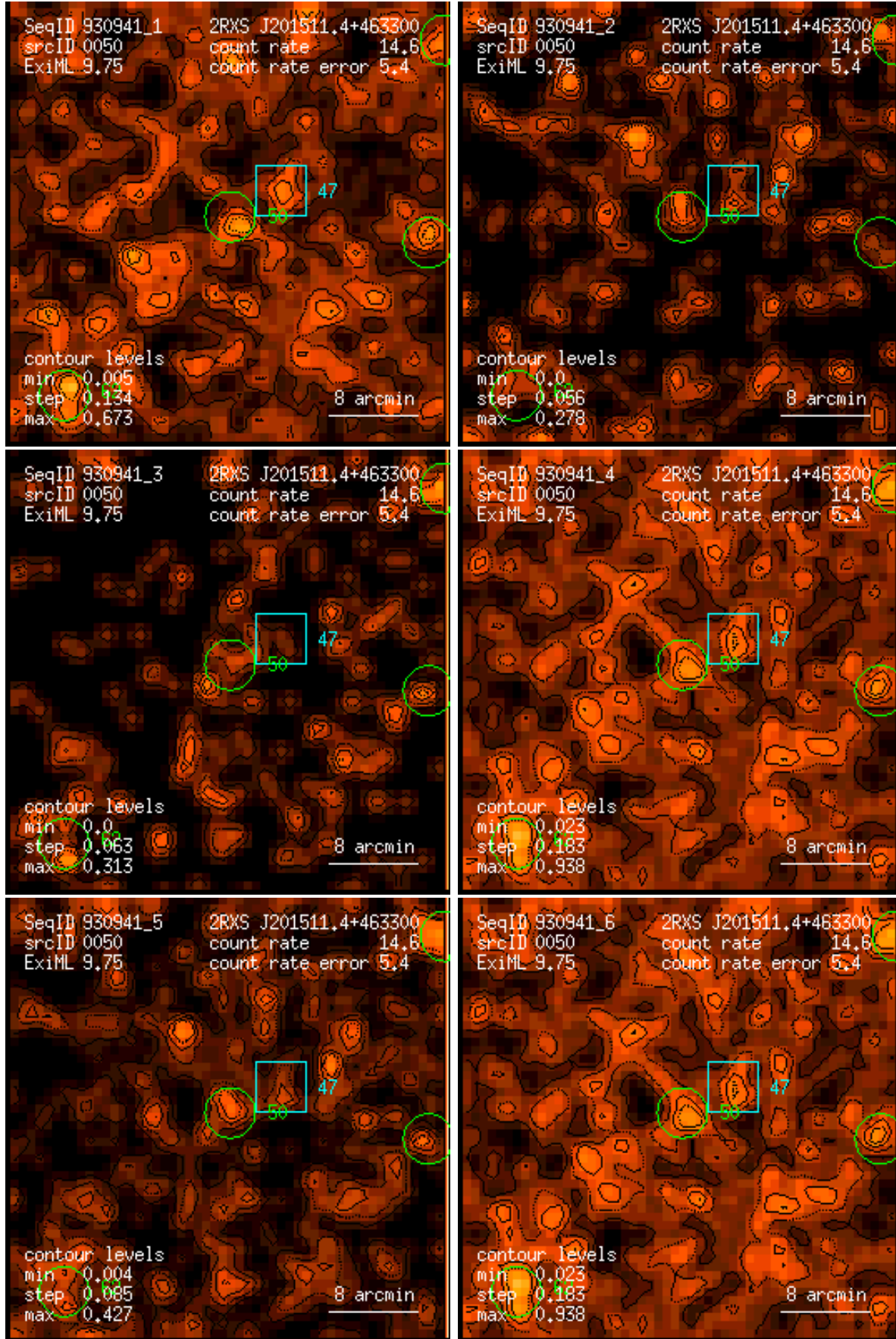
Figure 50: RASS 930941: detection 0050: band rate images, Gaussian filter: (1) PSPC channels 11 – 41, (2) 52 – 90, (3) 91 – 201, (4) 11 – 235, (5) 52 – 201, (6) 11 – 201. Broad band rates in counts/ks. Band rate contour levels in counts/ks/arcmin 2 .
