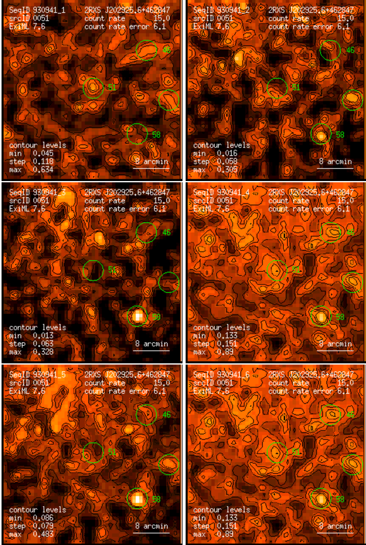
Figure 51: RASS 930941: detection 0051: band rate images, Gaussian filter: (1) PSPC channels 11 – 41, (2) 52 – 90, (3) 91 – 201, (4) 11 – 235, (5) 52 – 201, (6) 11 – 201. Broad band rates in counts/ks. Band rate contour levels in counts/ks/arcmin 2 .
