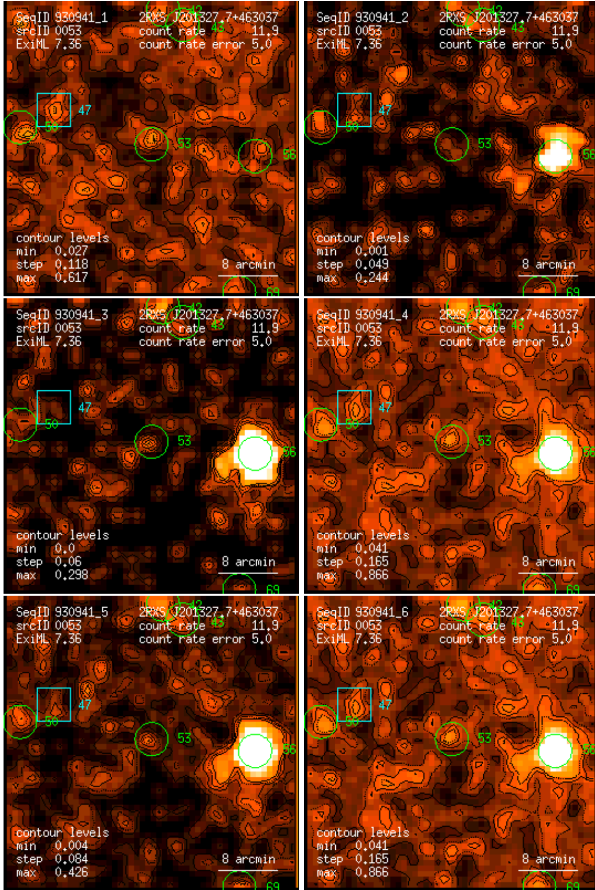
Figure 53: RASS 930941: detection 0053: band rate images, Gaussian filter: (1) PSPC channels 11 – 41, (2) 52 – 90, (3) 91 – 201, (4) 11 – 235, (5) 52 – 201, (6) 11 – 201. Broad band rates in counts/ks. Band rate contour levels in counts/ks/arcmin 2 .
