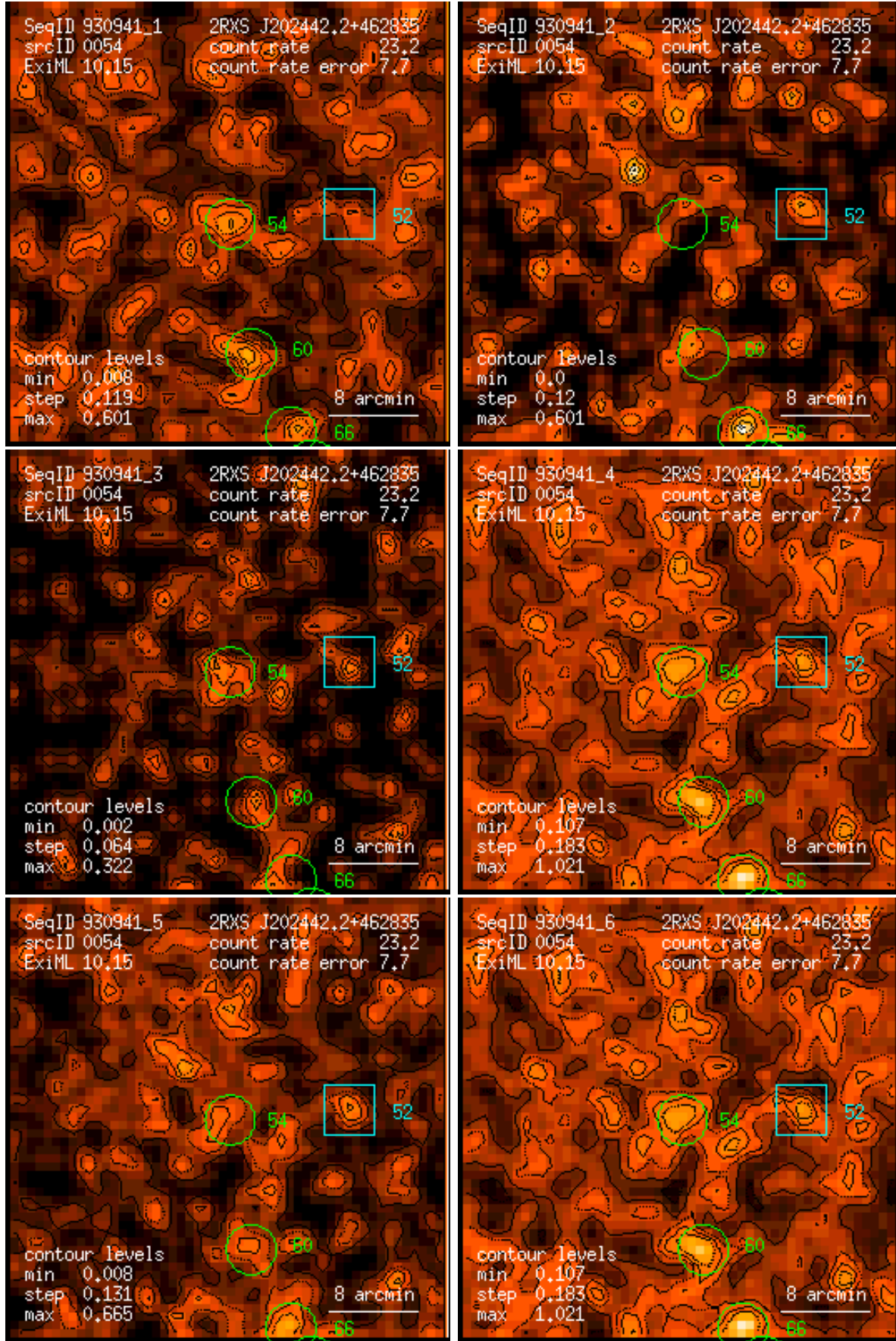
Figure 54: RASS 930941: detection 0054: band rate images, Gaussian filter: (1) PSPC channels 11 – 41, (2) 52 – 90, (3) 91 – 201, (4) 11 – 235, (5) 52 – 201, (6) 11 – 201. Broad band rates in counts/ks. Band rate contour levels in counts/ks/arcmin 2 .
