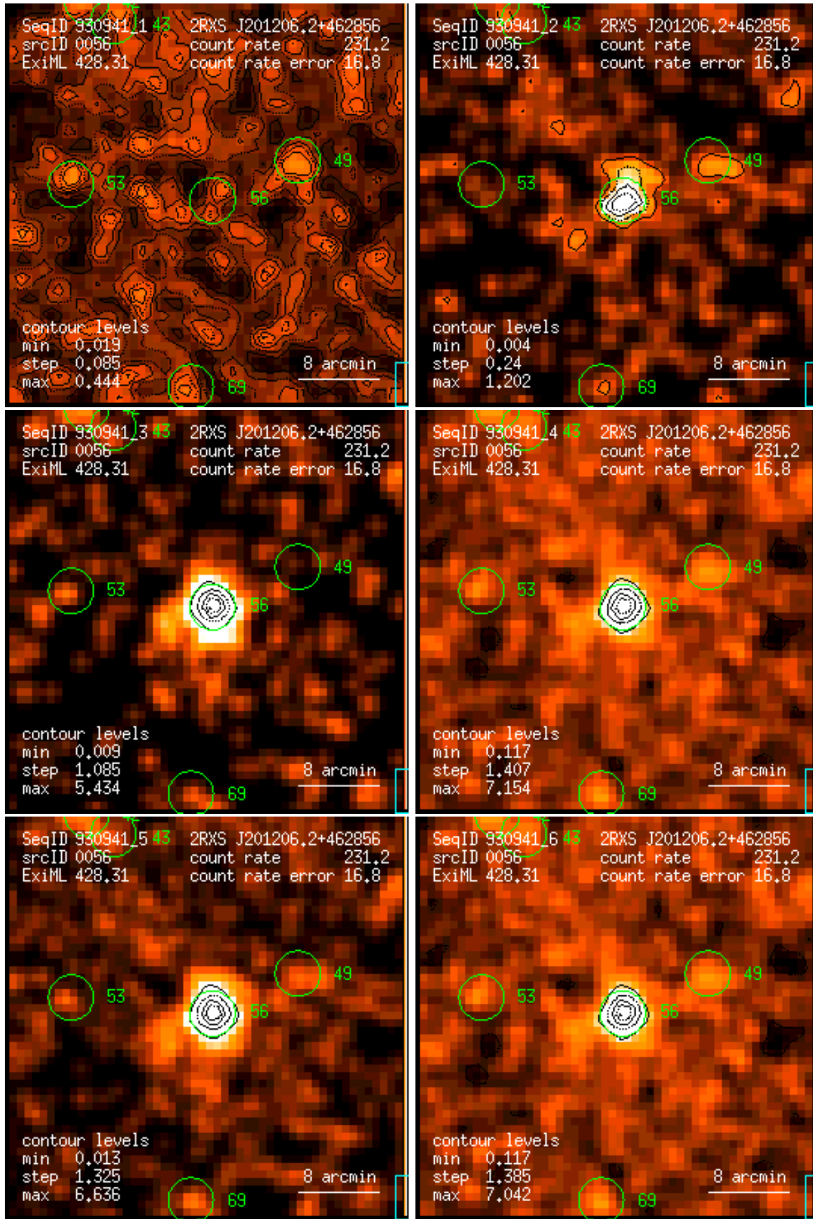
Figure 56: RASS 930941: detection 0056: band rate images, Gaussian filter: (1) PSPC channels 11 – 41, (2) 52 – 90, (3) 91 – 201, (4) 11 – 235, (5) 52 – 201, (6) 11 – 201. Broad band rates in counts/ks. Band rate contour levels in counts/ks/arcmin 2 .
