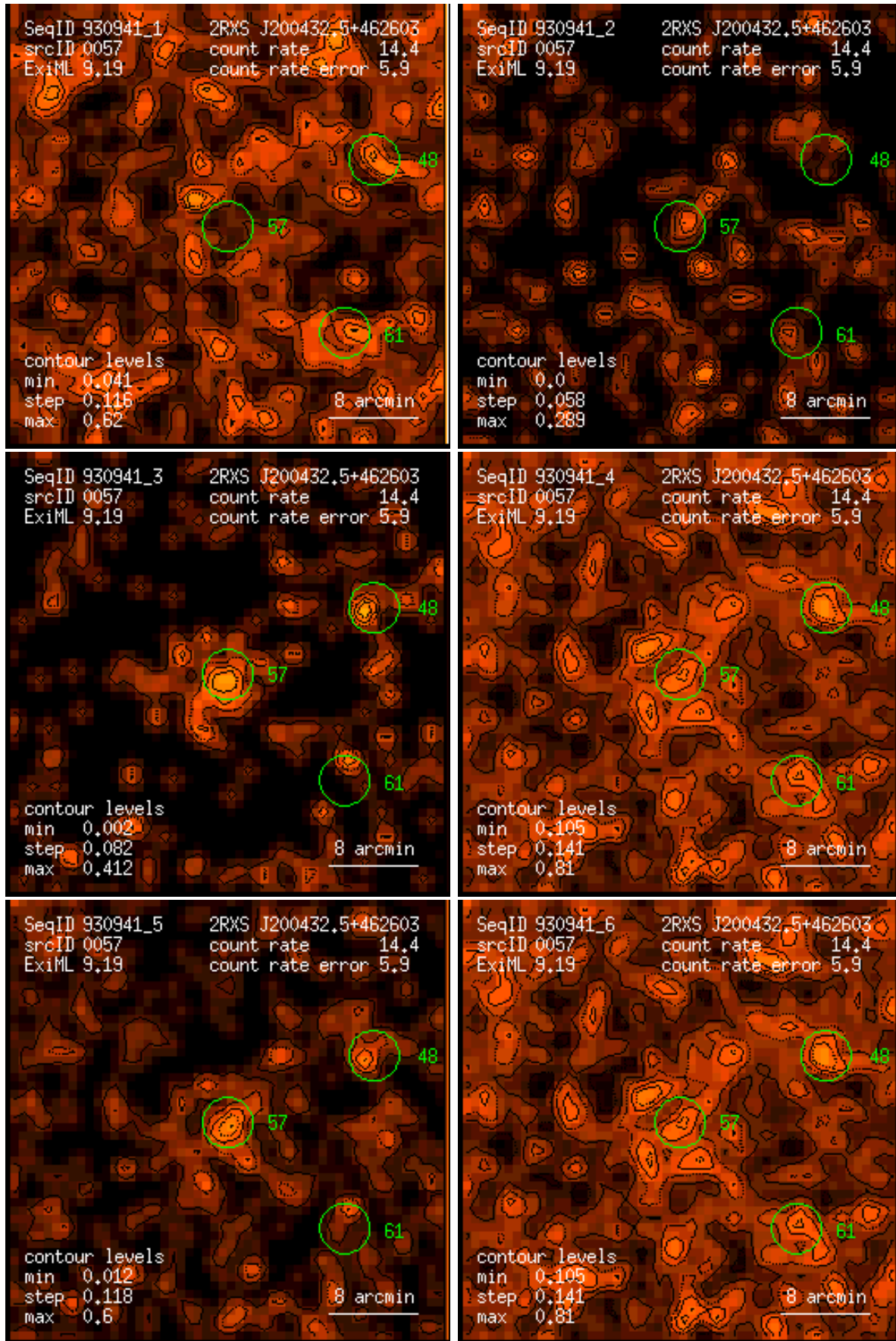
Figure 57: RASS 930941: detection 0057: band rate images, Gaussian filter: (1) PSPC channels 11 – 41, (2) 52 – 90, (3) 91 – 201, (4) 11 – 235, (5) 52 – 201, (6) 11 – 201. Broad band rates in counts/ks. Band rate contour levels in counts/ks/arcmin 2 .
