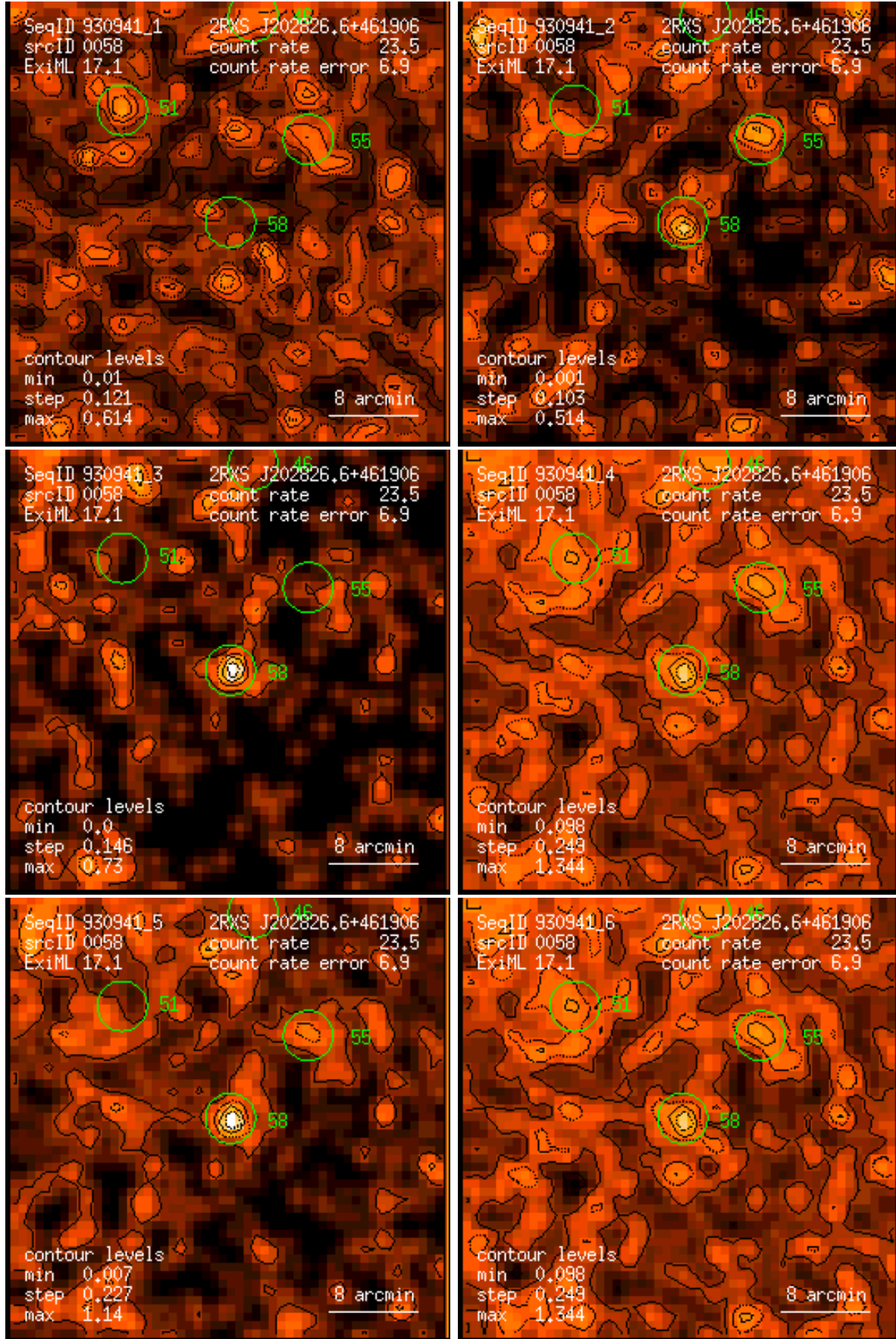
Figure 58: RASS 930941: detection 0058: band rate images, Gaussian filter: (1) PSPC channels 11 – 41, (2) 52 – 90, (3) 91 – 201, (4) 11 – 235, (5) 52 – 201, (6) 11 – 201. Broad band rates in counts/ks. Band rate contour levels in counts/ks/arcmin 2 .
