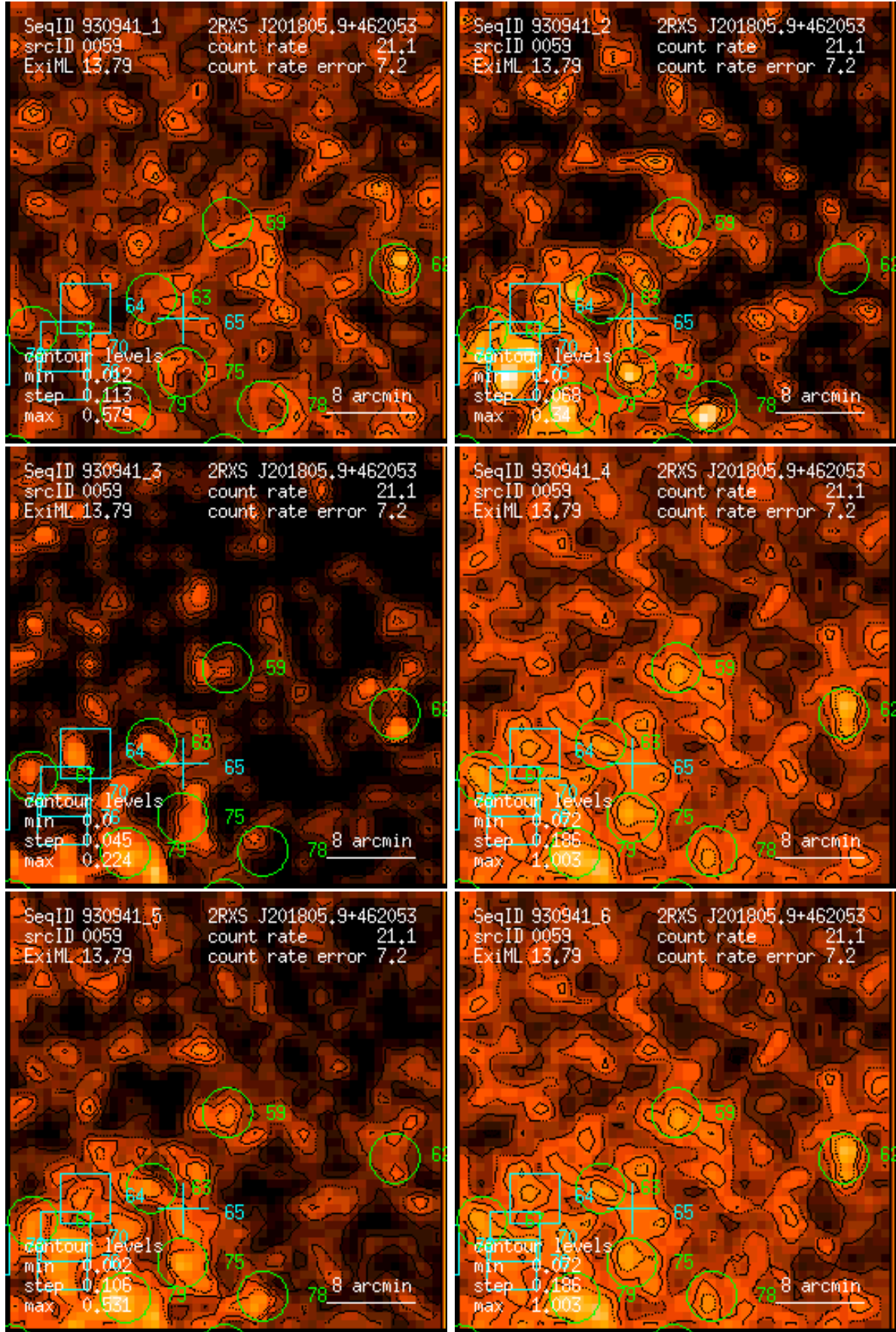
Figure 59: RASS 930941: detection 0059: band rate images, Gaussian filter: (1) PSPC channels 11 – 41, (2) 52 – 90, (3) 91 – 201, (4) 11 – 235, (5) 52 – 201, (6) 11 – 201. Broad band rates in counts/ks. Band rate contour levels in counts/ks/arcmin 2 .
