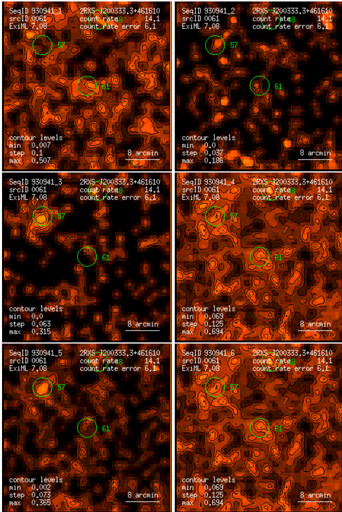
Figure 61: RASS 930941: detection 0061: band rate images, Gaussian filter: (1) PSPC channels 11 – 41, (2) 52 – 90, (3) 91 – 201, (4) 11 – 235, (5) 52 – 201, (6) 11 – 201. Broad band rates in counts/ks. Band rate contour levels in counts/ks/arcmin 2 .
