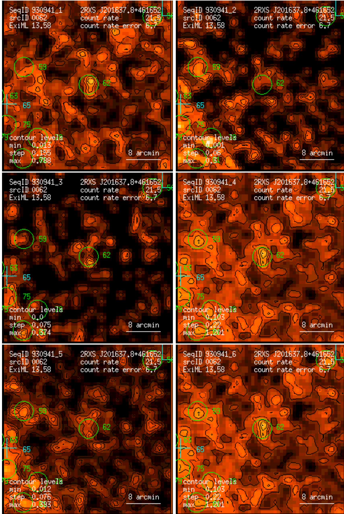
Figure 62: RASS 930941: detection 0062: band rate images, Gaussian filter: (1) PSPC channels 11 – 41, (2) 52 – 90, (3) 91 – 201, (4) 11 – 235, (5) 52 – 201, (6) 11 – 201. Broad band rates in counts/ks. Band rate contour levels in counts/ks/arcmin 2 .
