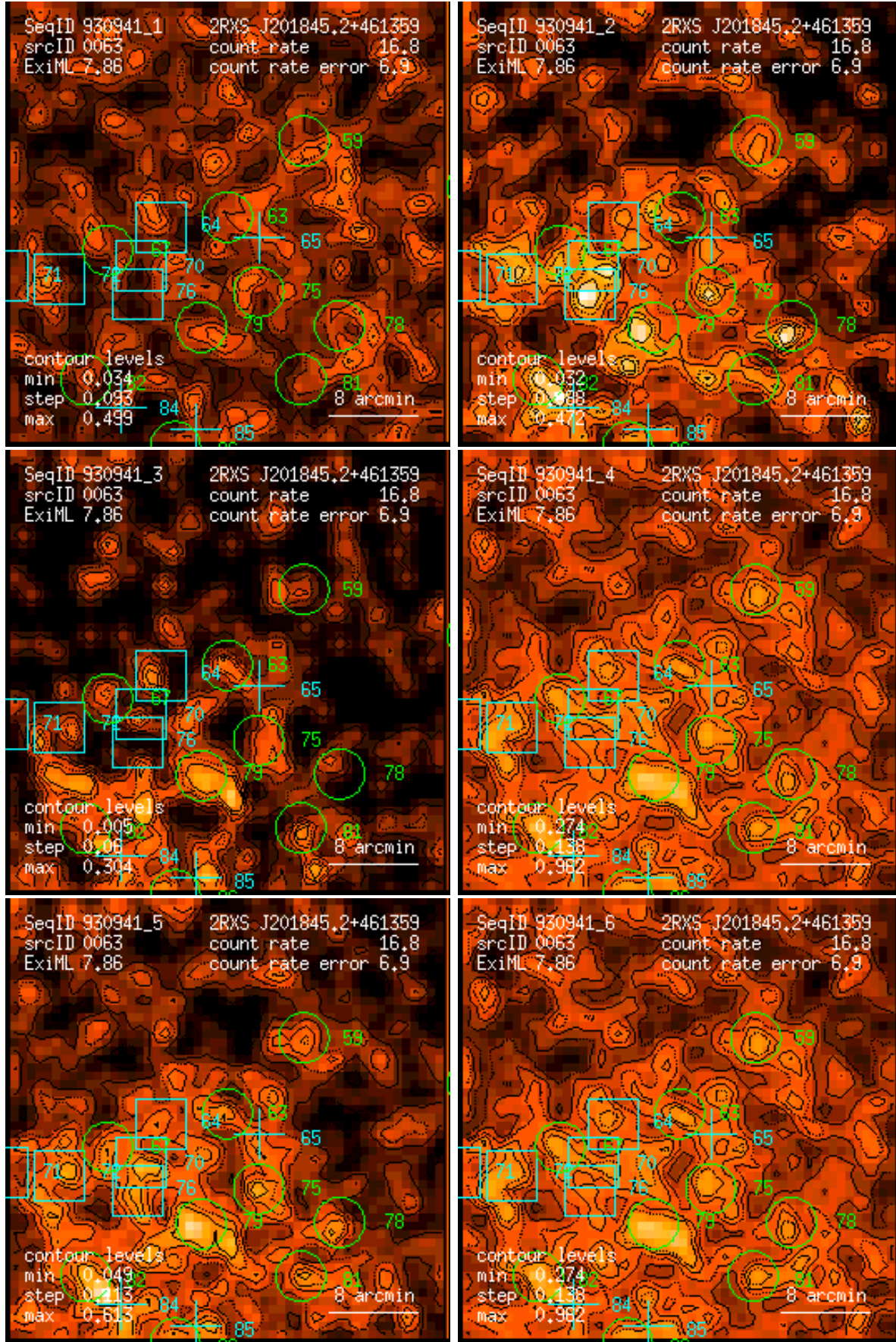
Figure 63: RASS 930941: detection 0063: band rate images, Gaussian filter: (1) PSPC channels 11 – 41, (2) 52 – 90, (3) 91 – 201, (4) 11 – 235, (5) 52 – 201, (6) 11 – 201. Broad band rates in counts/ks. Band rate contour levels in counts/ks/arcmin 2 .
