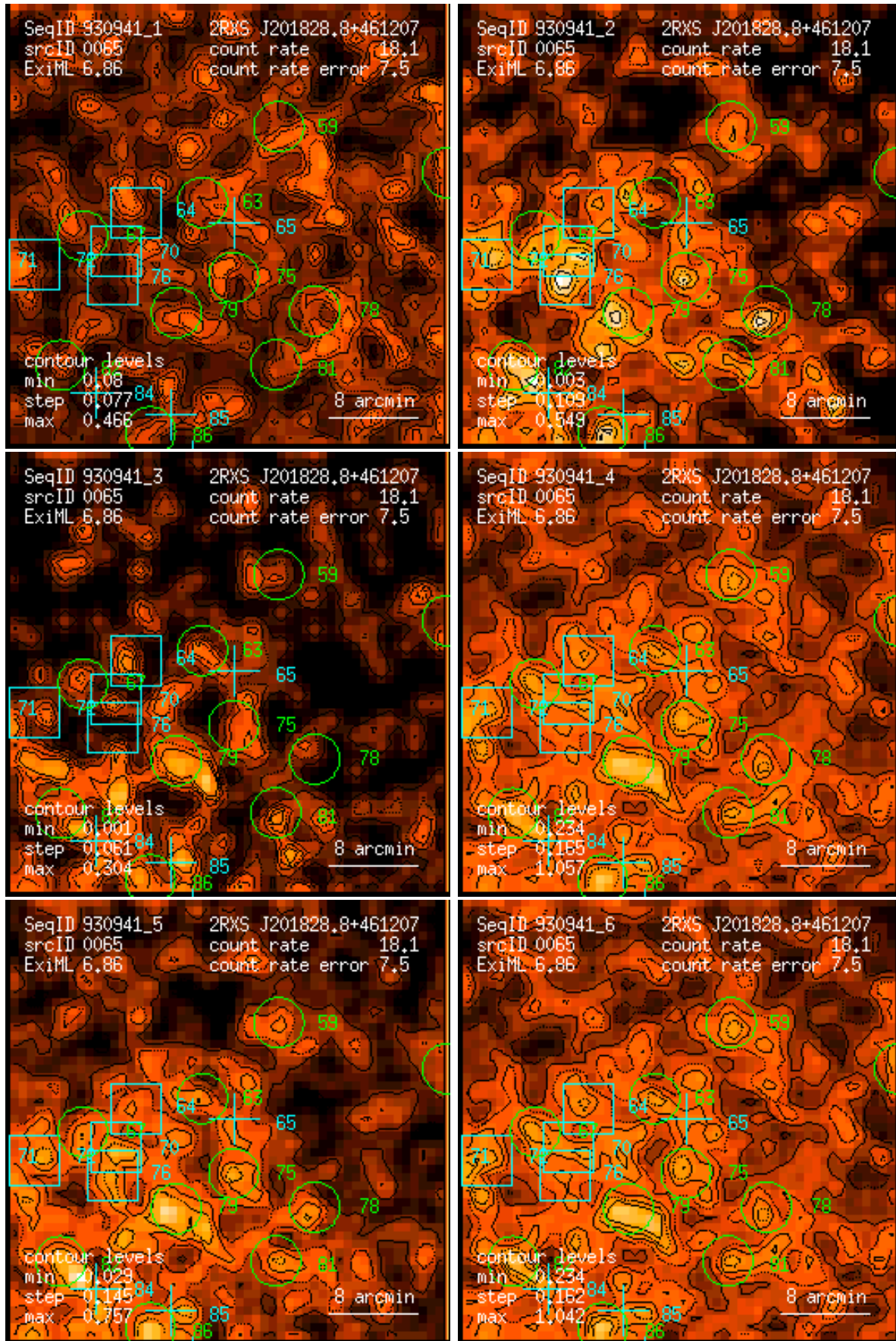
Figure 65: RASS 930941: detection 0065: band rate images, Gaussian filter: (1) PSPC channels 11 – 41, (2) 52 – 90, (3) 91 – 201, (4) 11 – 235, (5) 52 – 201, (6) 11 – 201. Broad band rates in counts/ks. Band rate contour levels in counts/ks/arcmin 2 .
