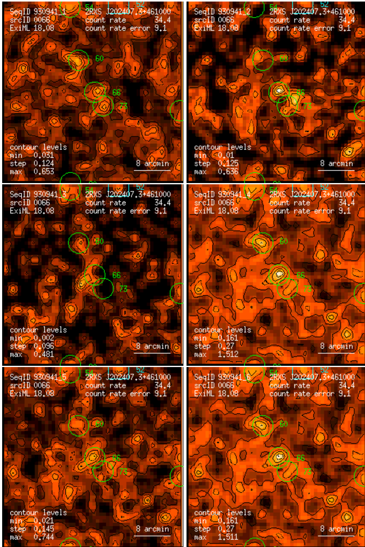
Figure 66: RASS 930941: detection 0066: band rate images, Gaussian filter: (1) PSPC channels 11 – 41, (2) 52 – 90, (3) 91 – 201, (4) 11 – 235, (5) 52 – 201, (6) 11 – 201. Broad band rates in counts/ks. Band rate contour levels in counts/ks/arcmin 2 .
