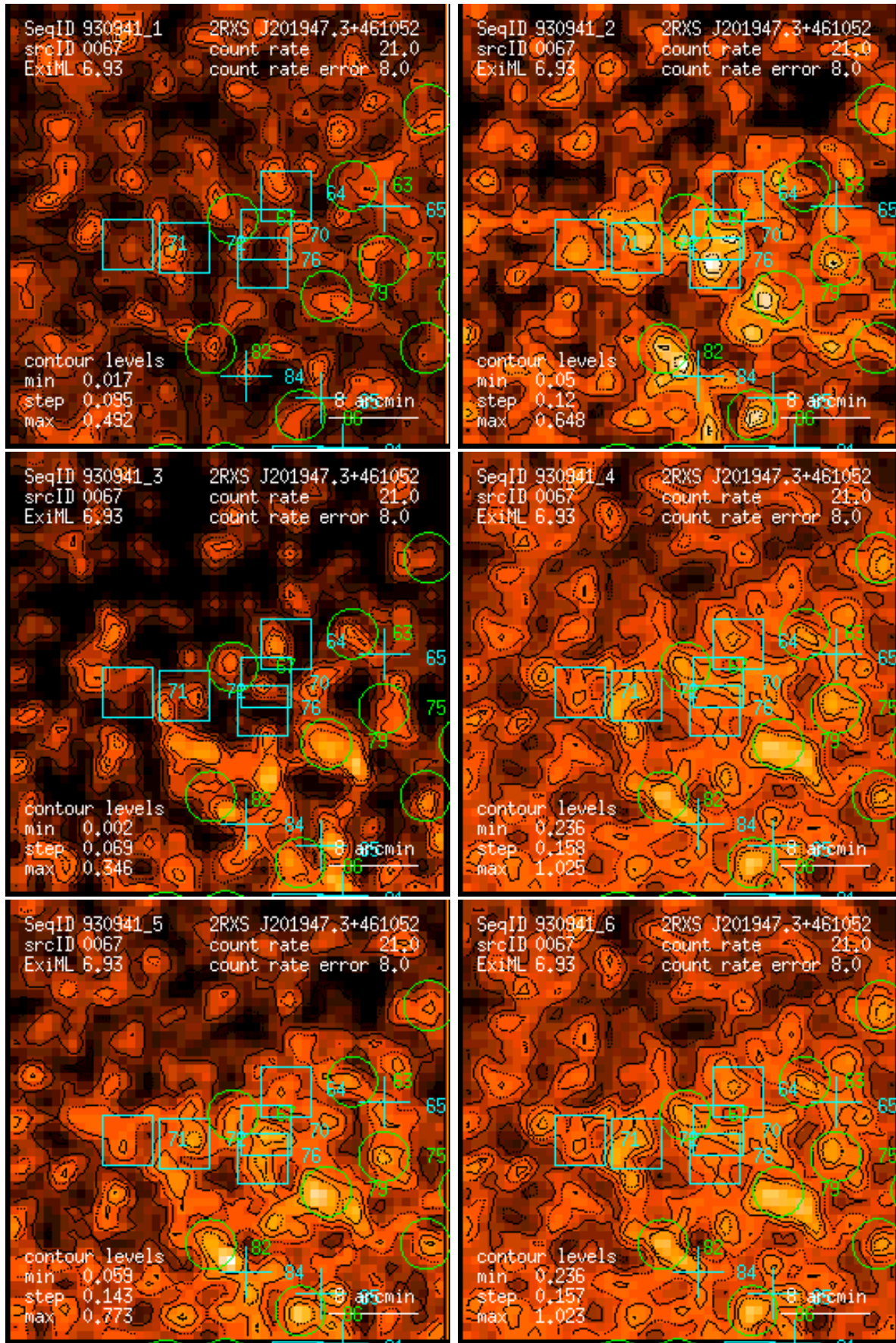
Figure 67: RASS 930941: detection 0067: band rate images, Gaussian filter: (1) PSPC channels 11 – 41, (2) 52 – 90, (3) 91 – 201, (4) 11 – 235, (5) 52 – 201, (6) 11 – 201. Broad band rates in counts/ks. Band rate contour levels in counts/ks/arcmin 2 .
