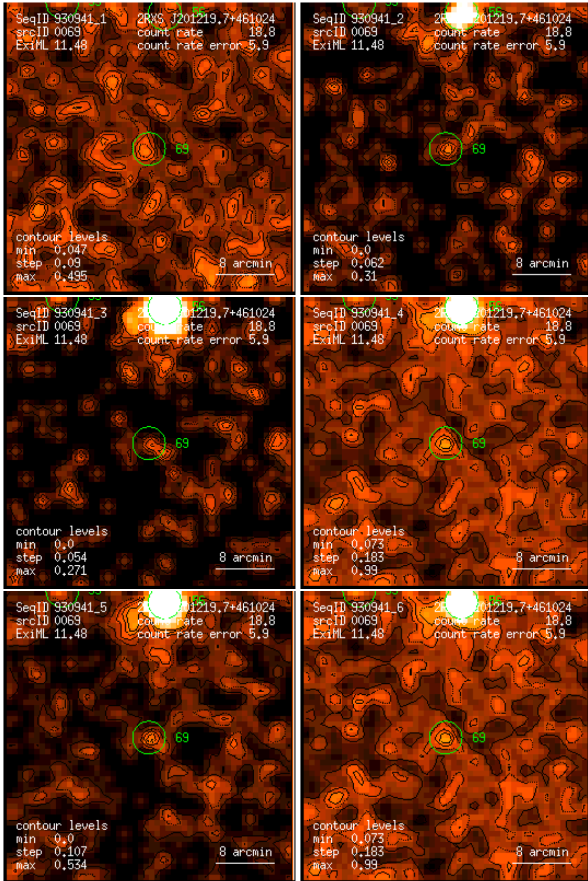
Figure 69: RASS 930941: detection 0069: band rate images, Gaussian filter: (1) PSPC channels 11 – 41, (2) 52 – 90, (3) 91 – 201, (4) 11 – 235, (5) 52 – 201, (6) 11 – 201. Broad band rates in counts/ks. Band rate contour levels in counts/ks/arcmin 2 .
