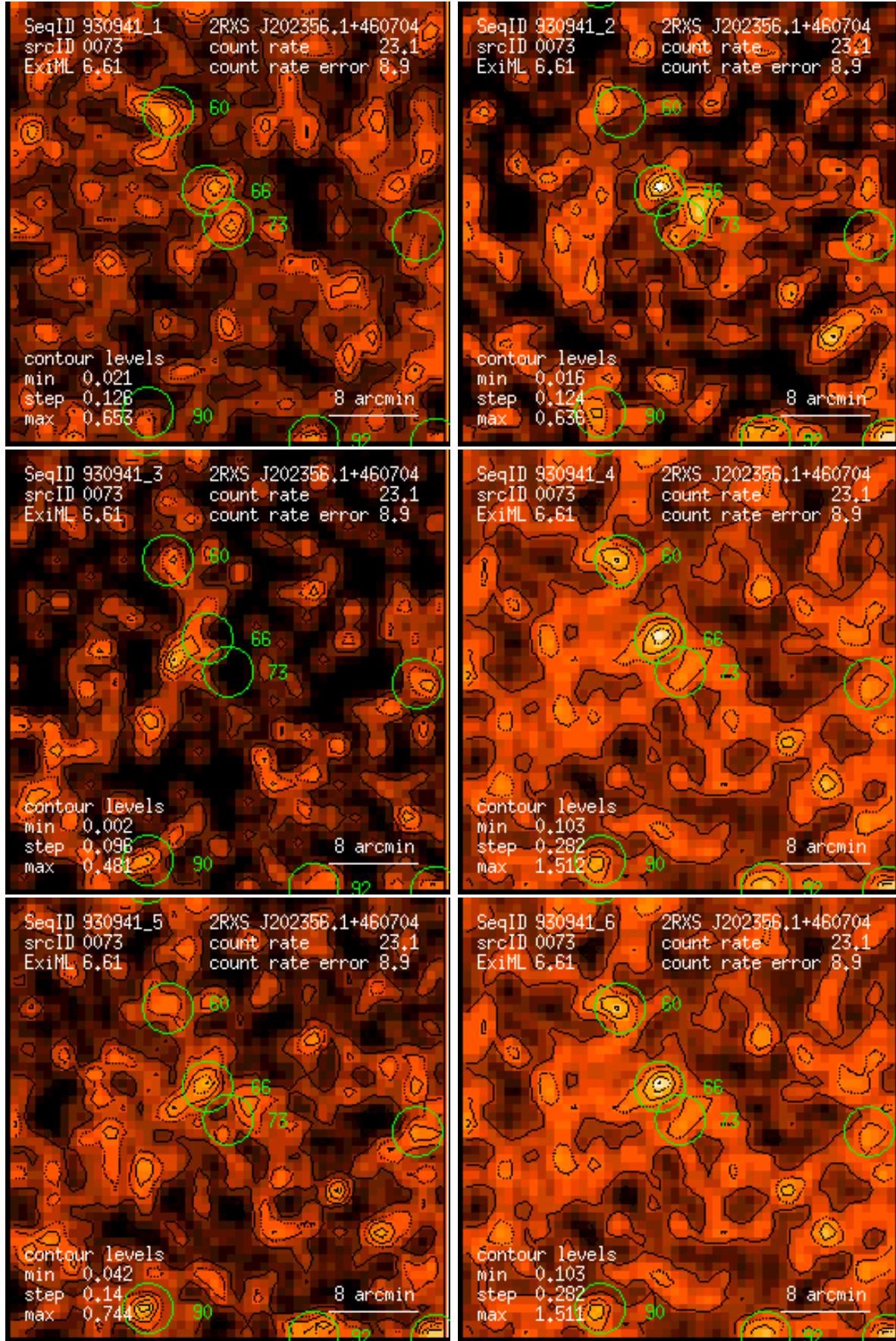
Figure 73: RASS 930941: detection 0073: band rate images, Gaussian filter: (1) PSPC channels 11 – 41, (2) 52 – 90, (3) 91 – 201, (4) 11 – 235, (5) 52 – 201, (6) 11 – 201. Broad band rates in counts/ks. Band rate contour levels in counts/ks/arcmin 2 .
