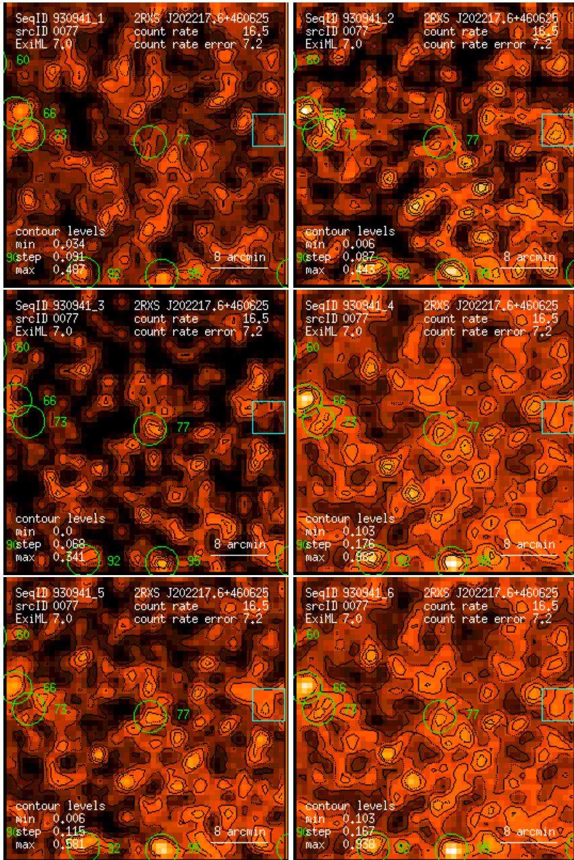
Figure 77: RASS 930941: detection 0077: band rate images, Gaussian filter: (1) PSPC channels 11 – 41, (2) 52 – 90, (3) 91 – 201, (4) 11 – 235, (5) 52 – 201, (6) 11 – 201. Broad band rates in counts/ks. Band rate contour levels in counts/ks/arcmin 2 .
