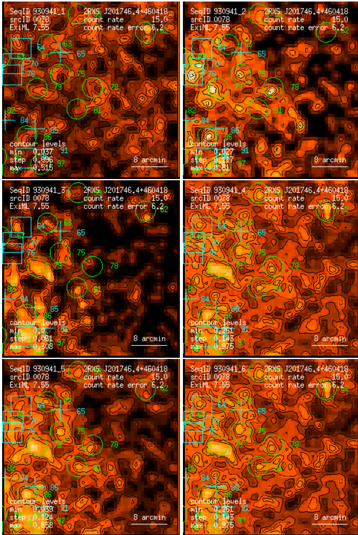
Figure 78: RASS 930941: detection 0078: band rate images, Gaussian filter: (1) PSPC channels 11 – 41, (2) 52 – 90, (3) 91 – 201, (4) 11 – 235, (5) 52 – 201, (6) 11 – 201. Broad band rates in counts/ks. Band rate contour levels in counts/ks/arcmin 2 .
