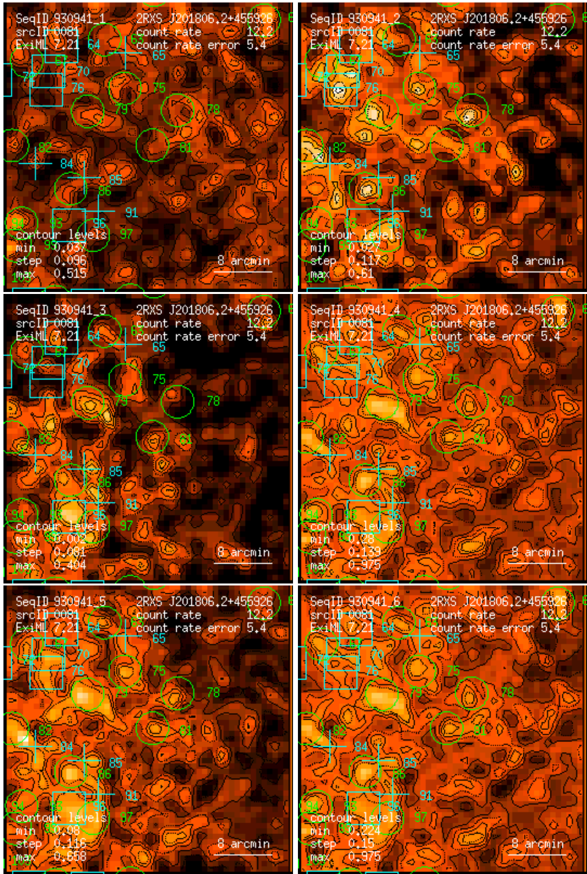
Figure 81: RASS 930941: detection 0081: band rate images, Gaussian filter: (1) PSPC channels 11 – 41, (2) 52 – 90, (3) 91 – 201, (4) 11 – 235, (5) 52 – 201, (6) 11 – 201. Broad band rates in counts/ks. Band rate contour levels in counts/ks/arcmin 2 .
