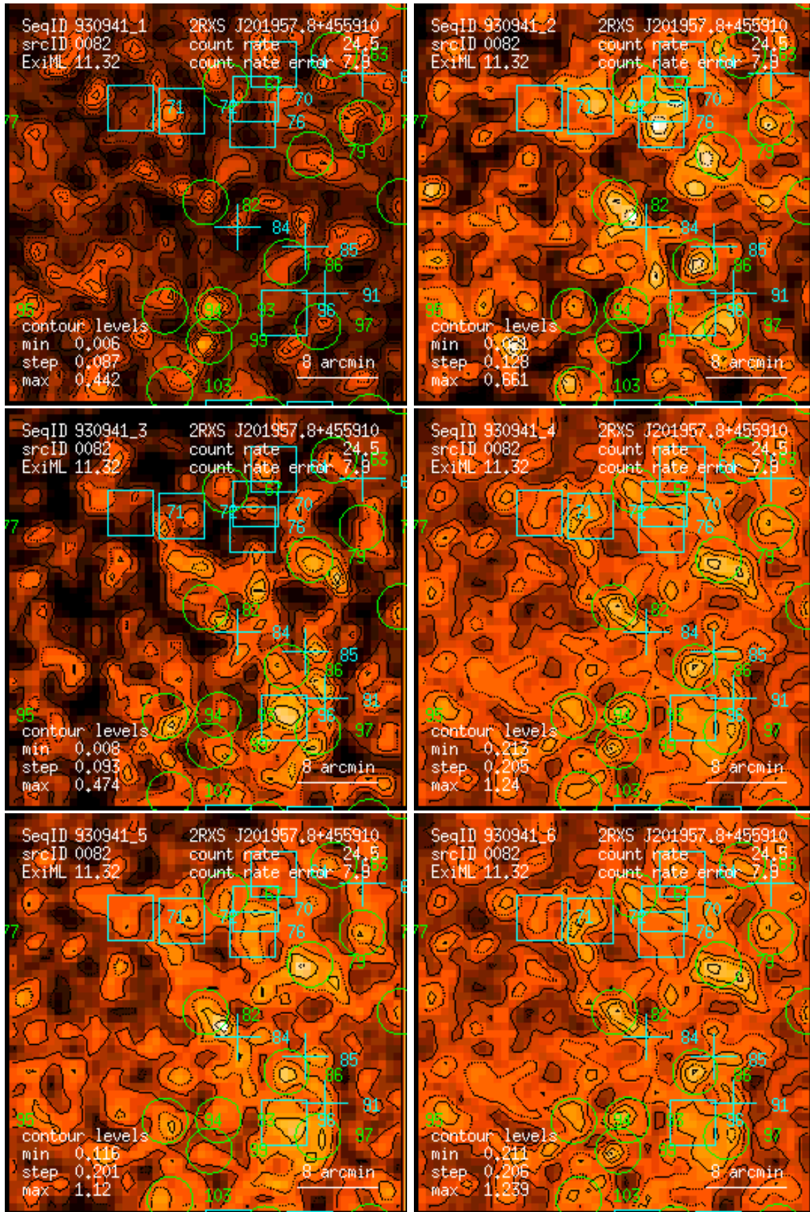
Figure 82: RASS 930941: detection 0082: band rate images, Gaussian filter: (1) PSPC channels 11 – 41, (2) 52 – 90, (3) 91 – 201, (4) 11 – 235, (5) 52 – 201, (6) 11 – 201. Broad band rates in counts/ks. Band rate contour levels in counts/ks/arcmin 2 .
