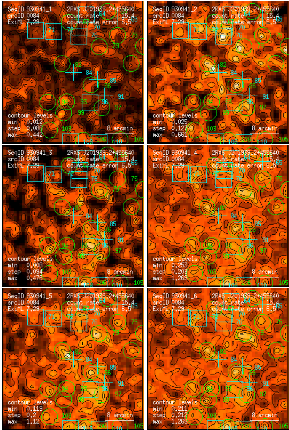
Figure 84: RASS 930941: detection 0084: band rate images, Gaussian filter: (1) PSPC channels 11 – 41, (2) 52 – 90, (3) 91 – 201, (4) 11 – 235, (5) 52 – 201, (6) 11 – 201. Broad band rates in counts/ks. Band rate contour levels in counts/ks/arcmin 2 .
