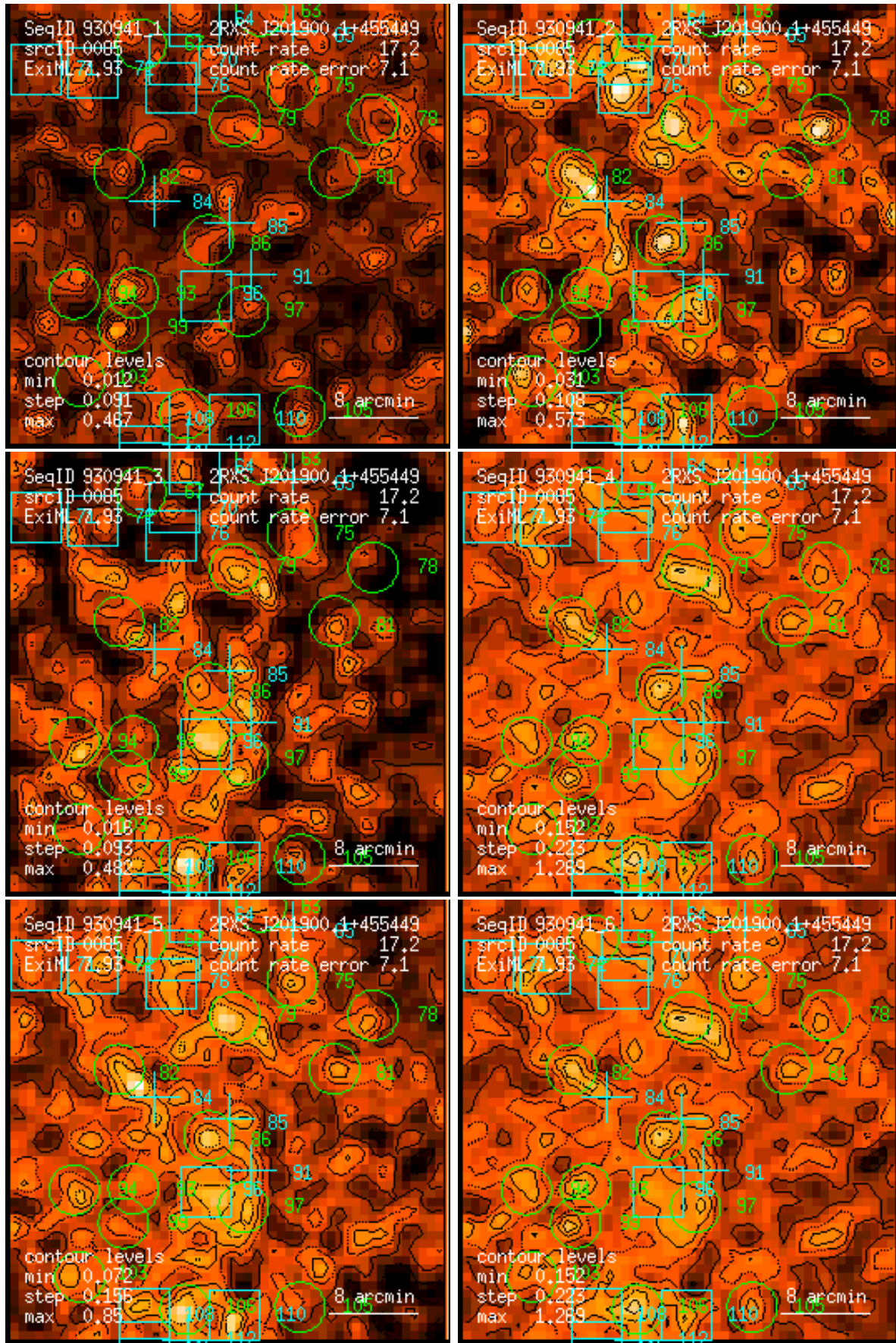
Figure 85: RASS 930941: detection 0085: band rate images, Gaussian filter: (1) PSPC channels 11 – 41, (2) 52 – 90, (3) 91 – 201, (4) 11 – 235, (5) 52 – 201, (6) 11 – 201. Broad band rates in counts/ks. Band rate contour levels in counts/ks/arcmin 2 .
