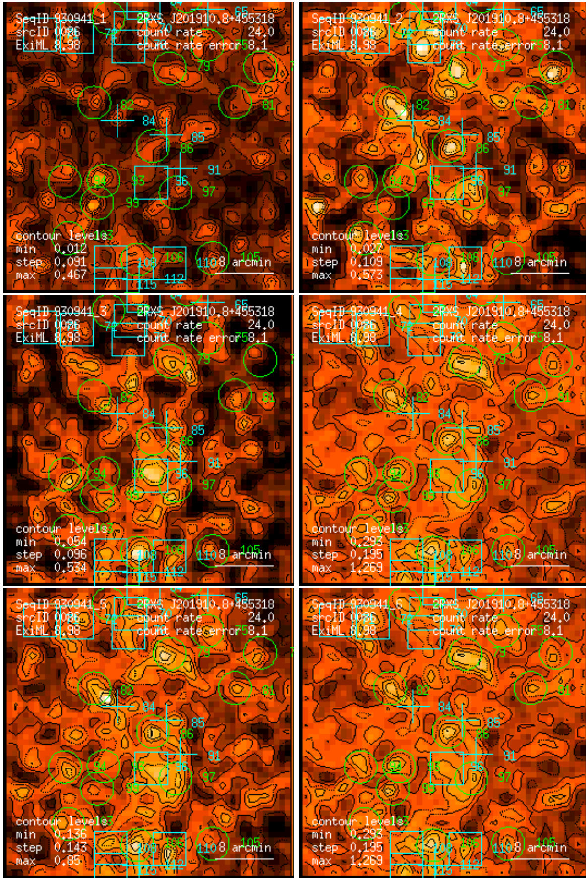
Figure 86: RASS 930941: detection 0086: band rate images, Gaussian filter: (1) PSPC channels 11 – 41, (2) 52 – 90, (3) 91 – 201, (4) 11 – 235, (5) 52 – 201, (6) 11 – 201. Broad band rates in counts/ks. Band rate contour levels in counts/ks/arcmin 2 .
