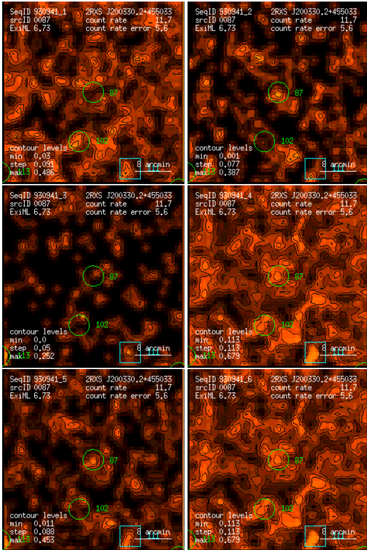
Figure 87: RASS 930941: detection 0087: band rate images, Gaussian filter: (1) PSPC channels 11 – 41, (2) 52 – 90, (3) 91 – 201, (4) 11 – 235, (5) 52 – 201, (6) 11 – 201. Broad band rates in counts/ks. Band rate contour levels in counts/ks/arcmin 2 .
