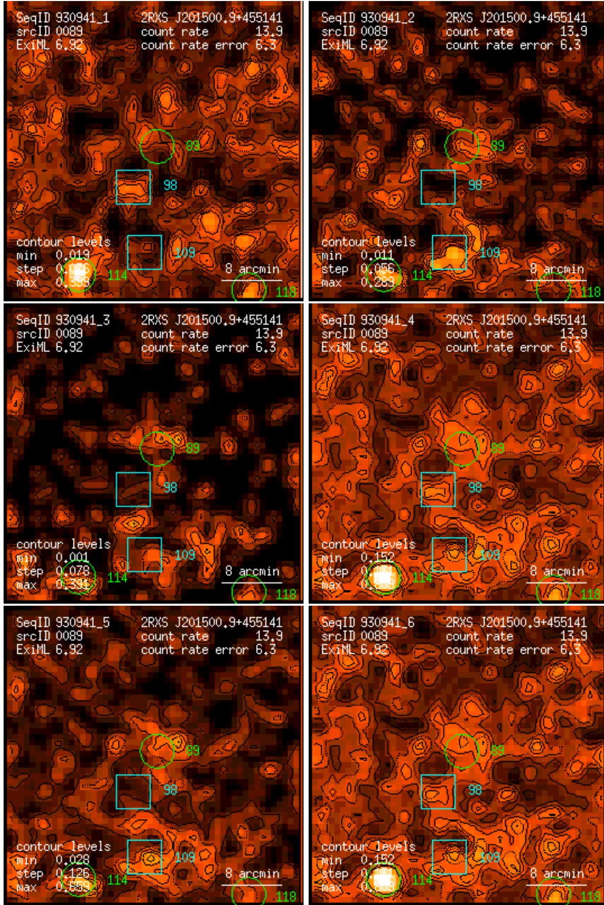
Figure 89: RASS 930941: detection 0089: band rate images, Gaussian filter: (1) PSPC channels 11 – 41, (2) 52 – 90, (3) 91 – 201, (4) 11 – 235, (5) 52 – 201, (6) 11 – 201. Broad band rates in counts/ks. Band rate contour levels in counts/ks/arcmin 2 .
