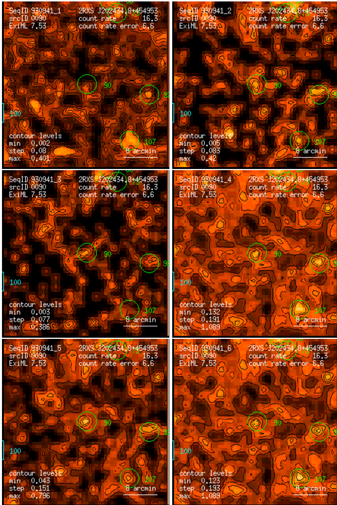
Figure 90: RASS 930941: detection 0090: band rate images, Gaussian filter: (1) PSPC channels 11 – 41, (2) 52 – 90, (3) 91 – 201, (4) 11 – 235, (5) 52 – 201, (6) 11 – 201. Broad band rates in counts/ks. Band rate contour levels in counts/ks/arcmin 2 .
