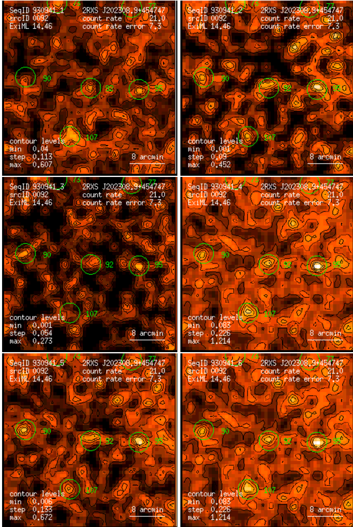
Figure 92: RASS 930941: detection 0092: band rate images, Gaussian filter: (1) PSPC channels 11 – 41, (2) 52 – 90, (3) 91 – 201, (4) 11 – 235, (5) 52 – 201, (6) 11 – 201. Broad band rates in counts/ks. Band rate contour levels in counts/ks/arcmin 2 .
