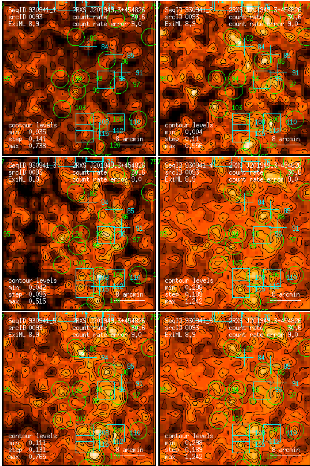
Figure 93: RASS 930941: detection 0093: band rate images, Gaussian filter: (1) PSPC channels 11 – 41, (2) 52 – 90, (3) 91 – 201, (4) 11 – 235, (5) 52 – 201, (6) 11 – 201. Broad band rates in counts/ks. Band rate contour levels in counts/ks/arcmin 2 .
