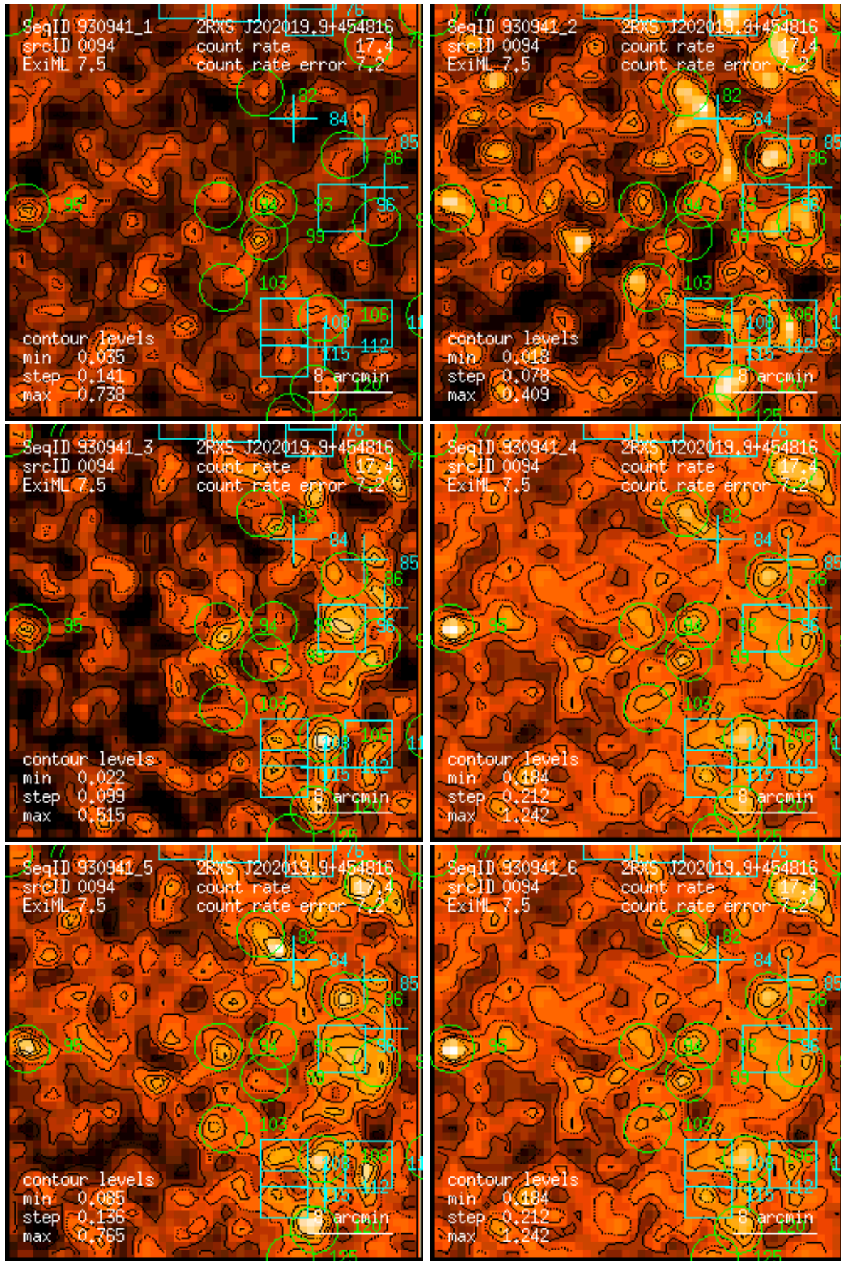
Figure 94: RASS 930941: detection 0094: band rate images, Gaussian filter: (1) PSPC channels 11 – 41, (2) 52 – 90, (3) 91 – 201, (4) 11 – 235, (5) 52 – 201, (6) 11 – 201. Broad band rates in counts/ks. Band rate contour levels in counts/ks/arcmin 2 .
