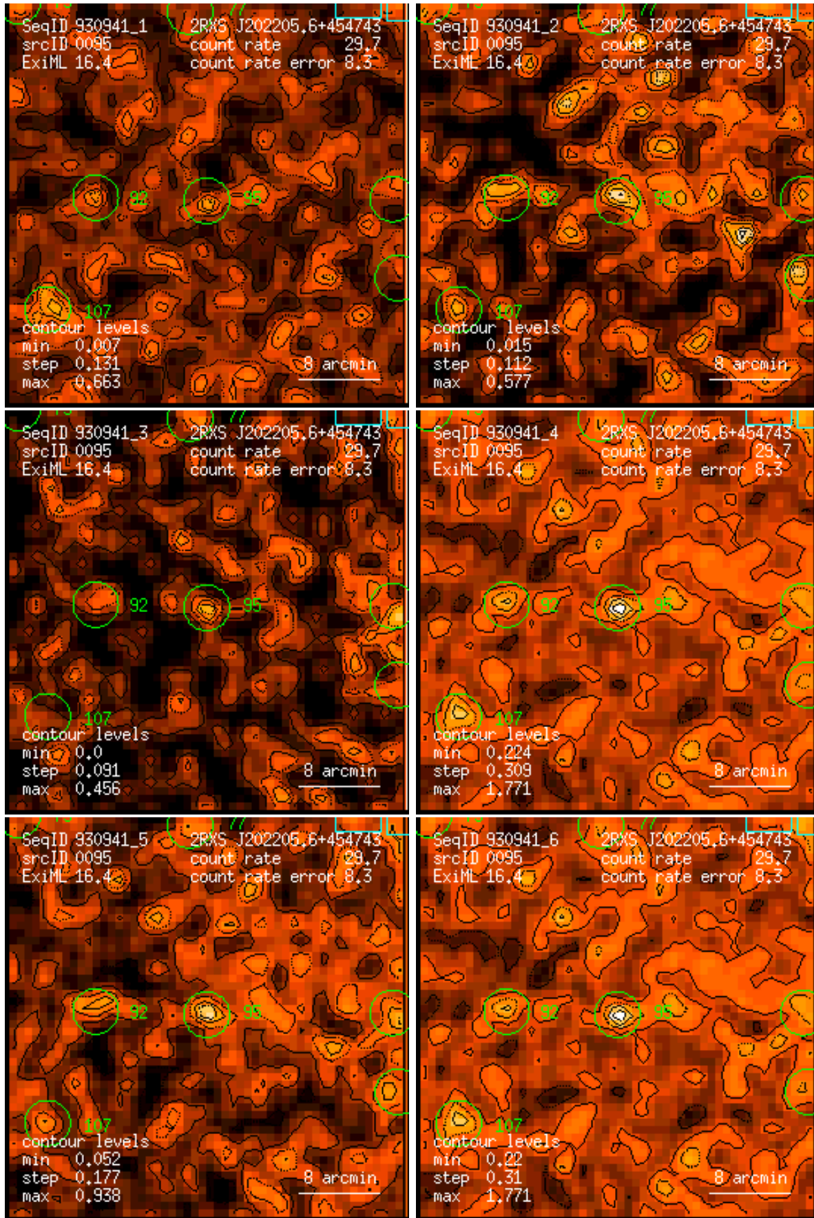
Figure 95: RASS 930941: detection 0095: band rate images, Gaussian filter: (1) PSPC channels 11 – 41, (2) 52 – 90, (3) 91 – 201, (4) 11 – 235, (5) 52 – 201, (6) 11 – 201. Broad band rates in counts/ks. Band rate contour levels in counts/ks/arcmin 2 .
