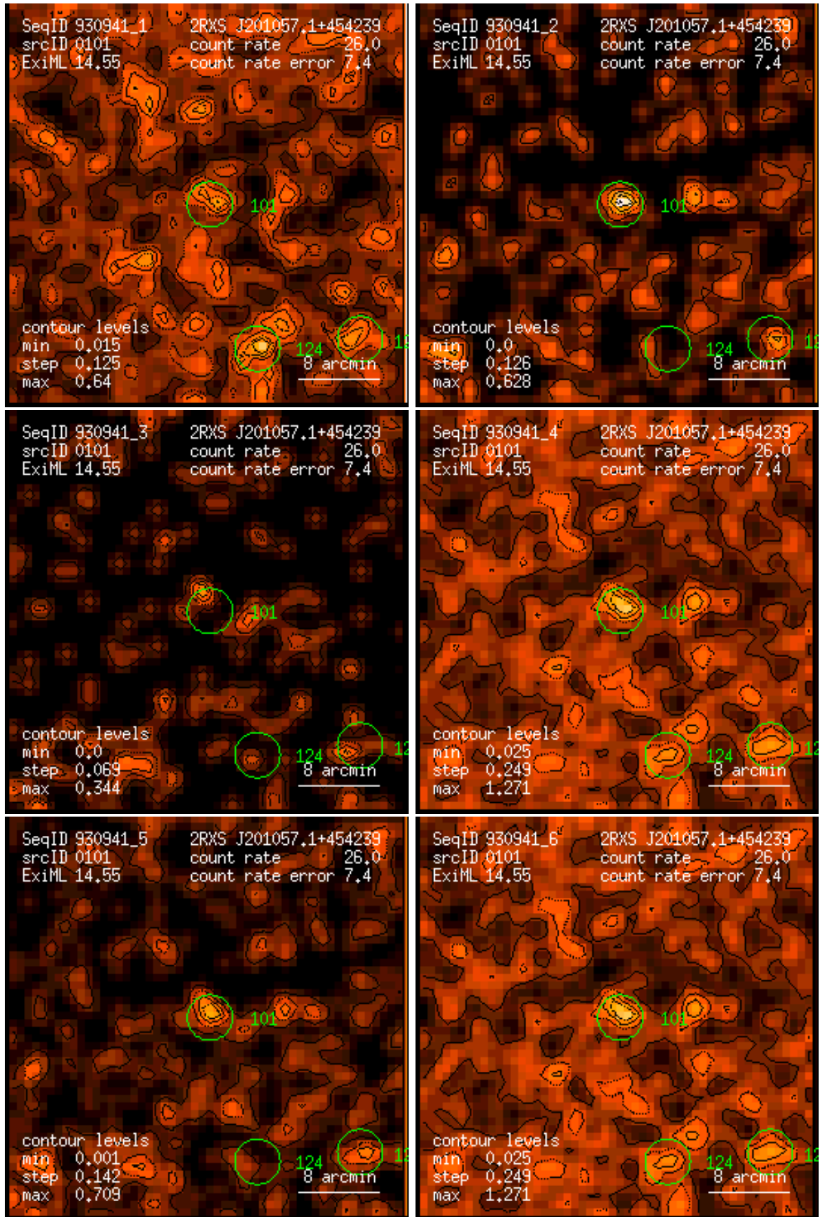
Figure 101: RASS 930941: detection 0101: band rate images, Gaussian filter: (1) PSPC channels 11 – 41, (2) 52 – 90, (3) 91 – 201, (4) 11 – 235, (5) 52 – 201, (6) 11 – 201. Broad band rates in counts/ks. Band rate contour levels in counts/ks/arcmin 2 .
